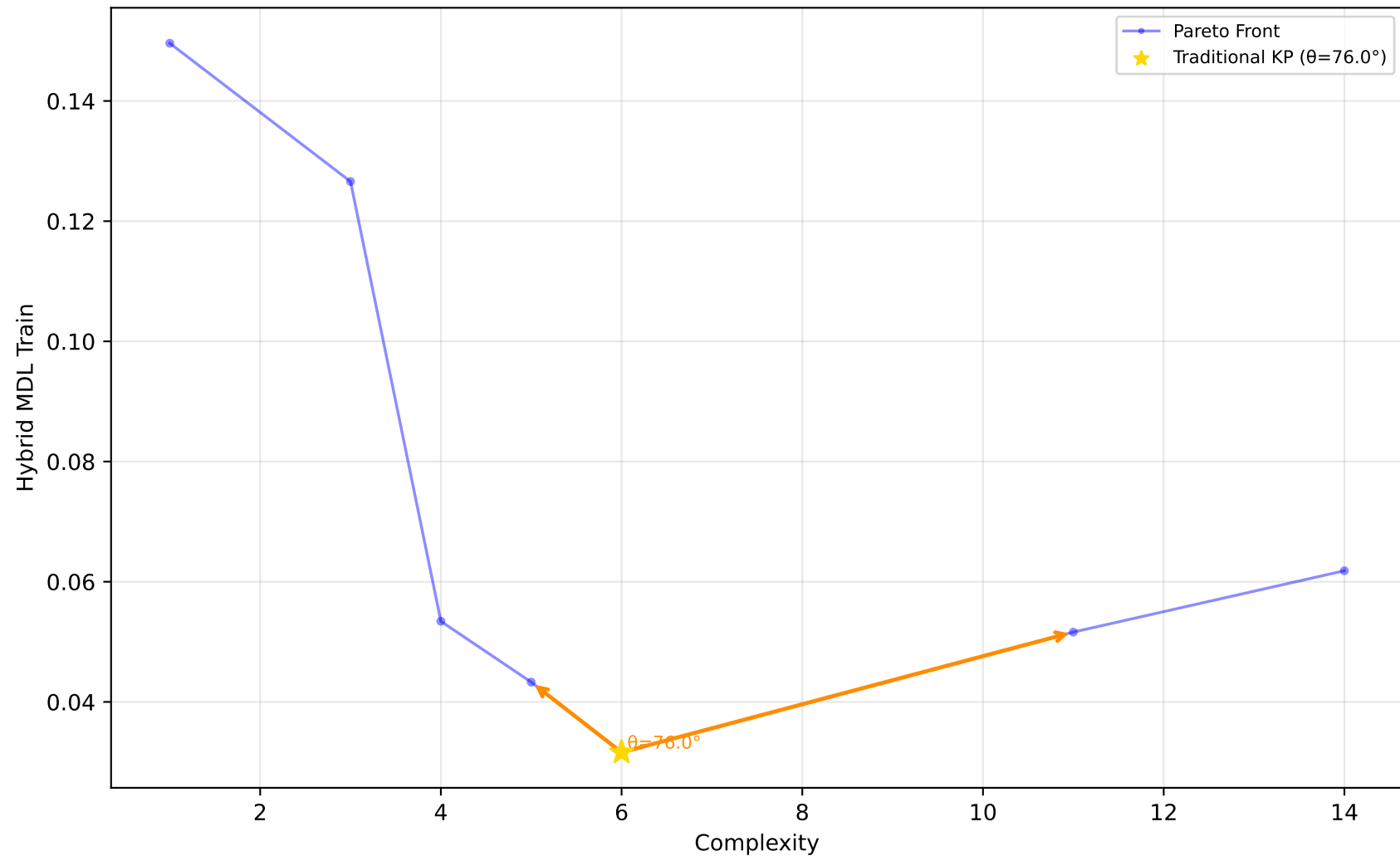
523_analcatdata_neavote - Run 7 - SVP - Hybrid MDL Train \lambda_1=0.00, \lambda_2=0.20, \lambda_3=0.00 | Difficulty: 1.00 | Method: hmr
