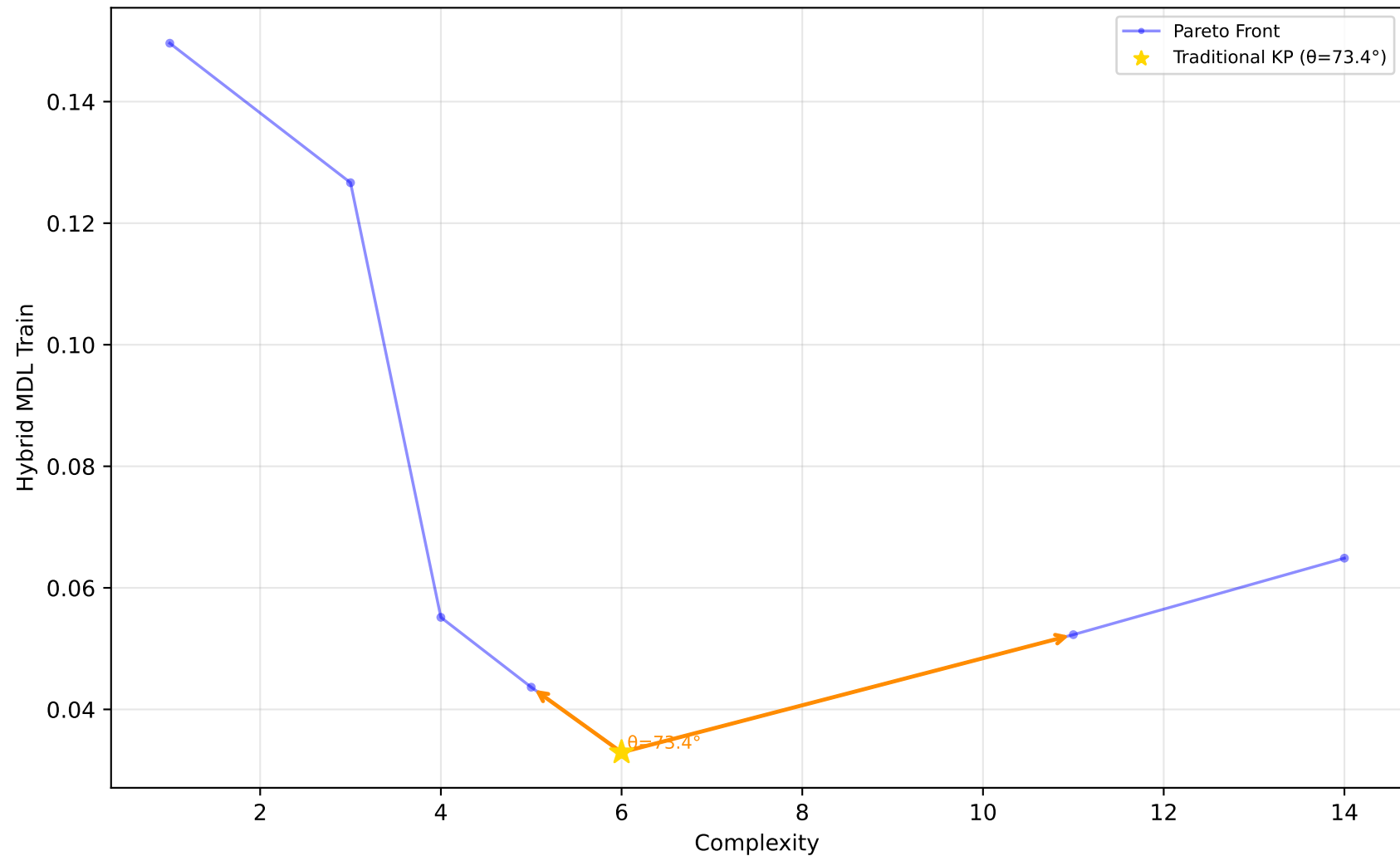
523_analcatdata_neavote - Run 7 - SVP - Hybrid MDL Train \lambda_1=0.00, \lambda_2=0.90, \lambda_3=0.00 | Difficulty: 1.00 | Method: hmr
