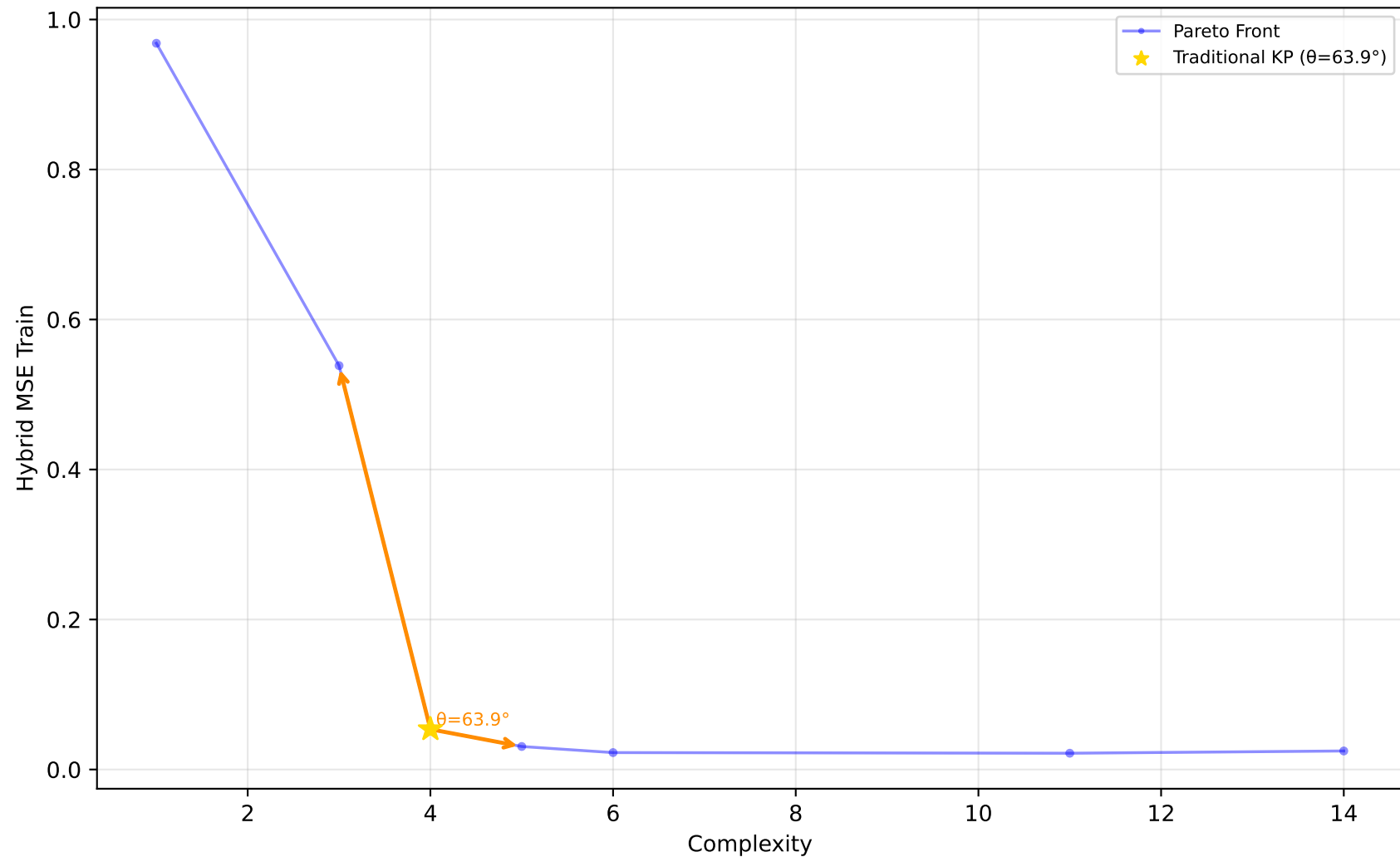
523_analcatdata_neavote - Run 7 - SVP - Hybrid MSE Train \lambda_1=0.00, \lambda_2=0.90, \lambda_3=0.00 | Difficulty: 1.00 | Method: hmr
