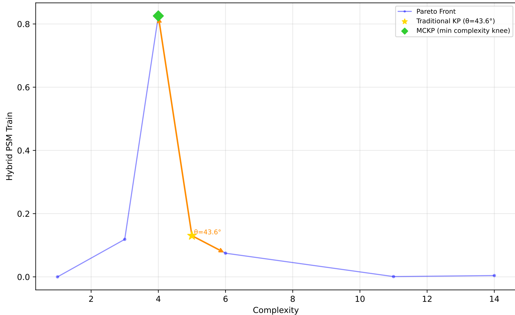
523_analcatdata_neavote - Run 7 - SVP - Hybrid PSM Train \lambda_1=0.00, \lambda_2=0.90, \lambda_3=0.00 | Difficulty: 1.00 | Method: hmr
