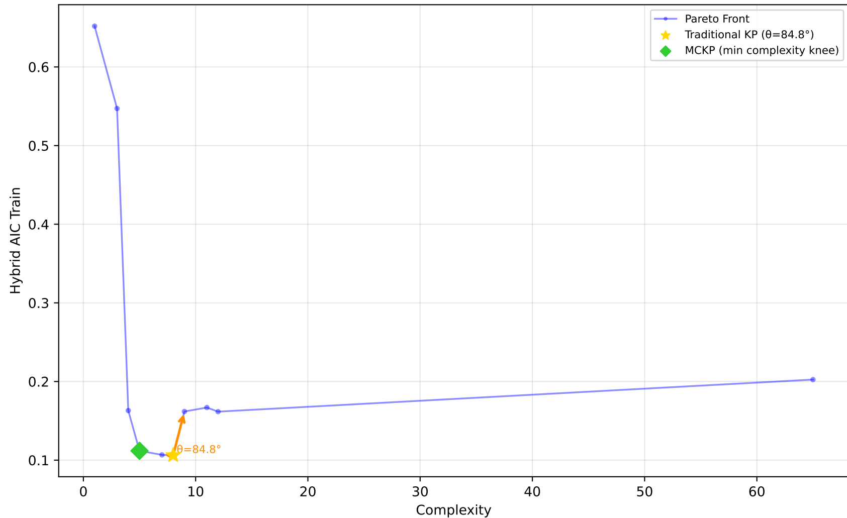
523_analcatdata_neavote - Run 8 - MVP - Hybrid AIC Train \lambda_1=0.00, \lambda_2=0.10, \lambda_3=0.00 | Difficulty: 1.00 | Method: hmr
