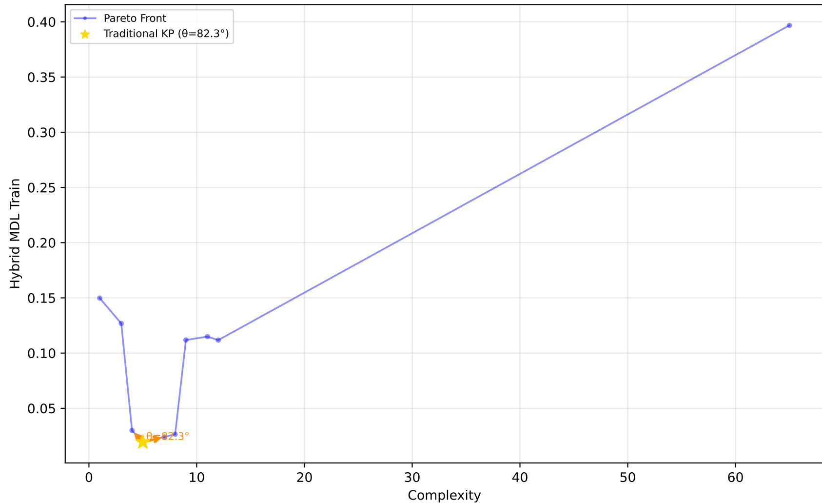
523_analcatdata_neavote - Run 8 - MVP - Hybrid MDL Train \lambda_1=0.00, \lambda_2=0.10, \lambda_3=0.00 | Difficulty: 1.00 | Method: hmr
