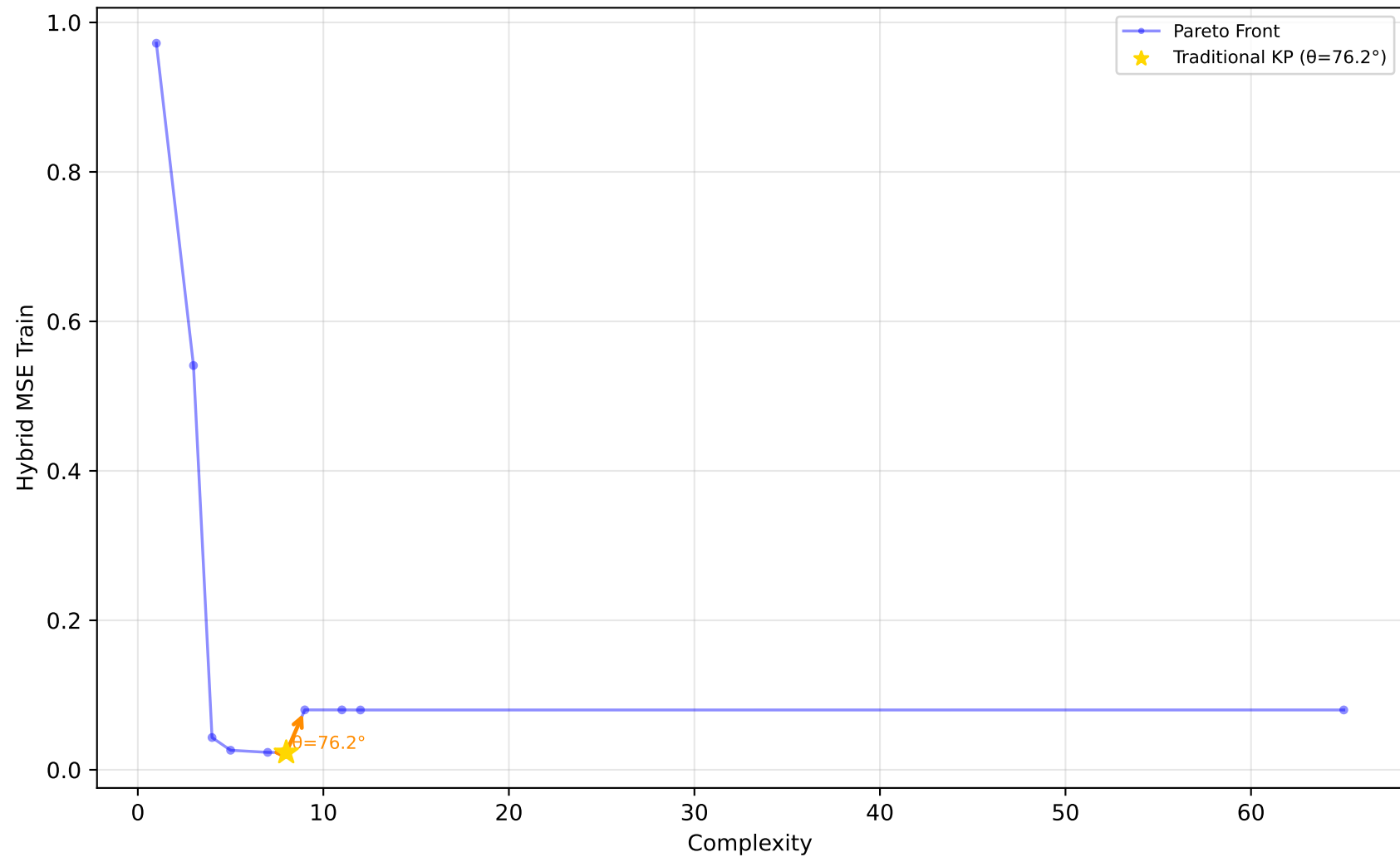
523_analcatdata_neavote - Run 8 - MVP - Hybrid MSE Train \lambda_1=0.00, \lambda_2=0.10, \lambda_3=0.00 | Difficulty: 1.00 | Method: hmr
