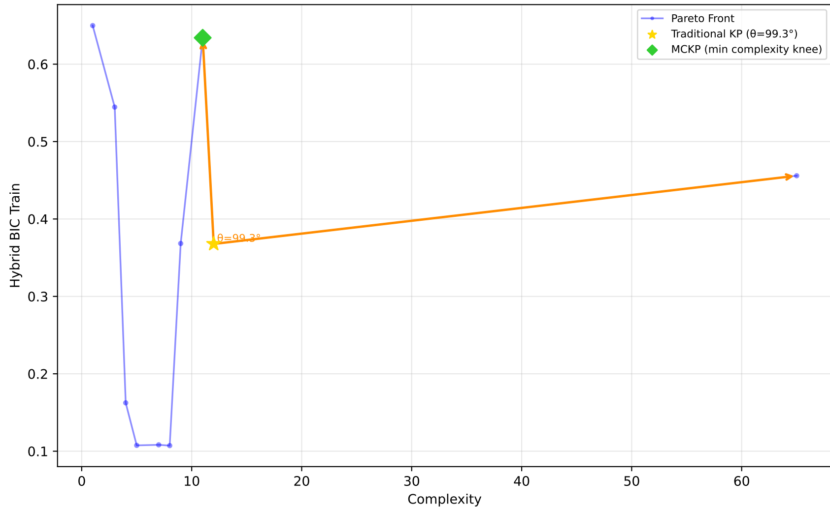
523_analcatdata_neavote - Run 8 - SVP - Hybrid BIC Train \lambda_1=0.00, \lambda_2=0.90, \lambda_3=0.00 | Difficulty: 1.00 | Method: hmr
