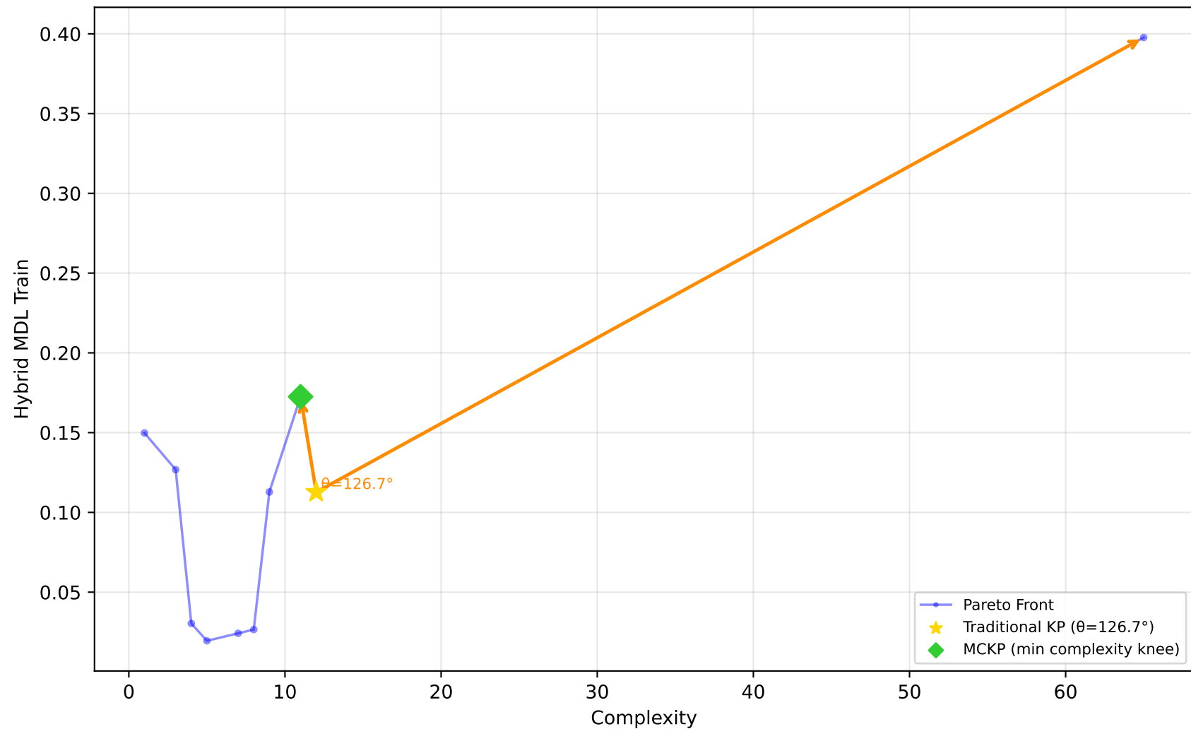
523_analcatdata_neavote - Run 8 - SVP - Hybrid MDL Train \lambda_1=0.00 , \lambda_2=0.20 , \lambda_3=0.00 | Difficulty: 1.00 | Method: hmr
