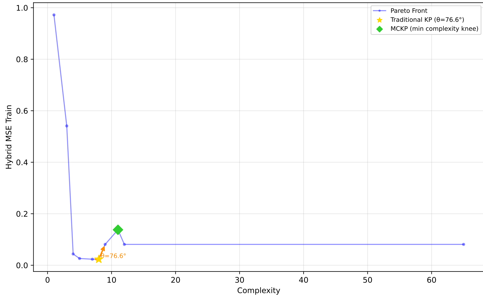
523_analcatdata_neavote - Run 8 - SVP - Hybrid MSE Train \lambda_1=0.00, \lambda_2=0.20, \lambda_3=0.00 | Difficulty: 1.00 | Method: hmr
