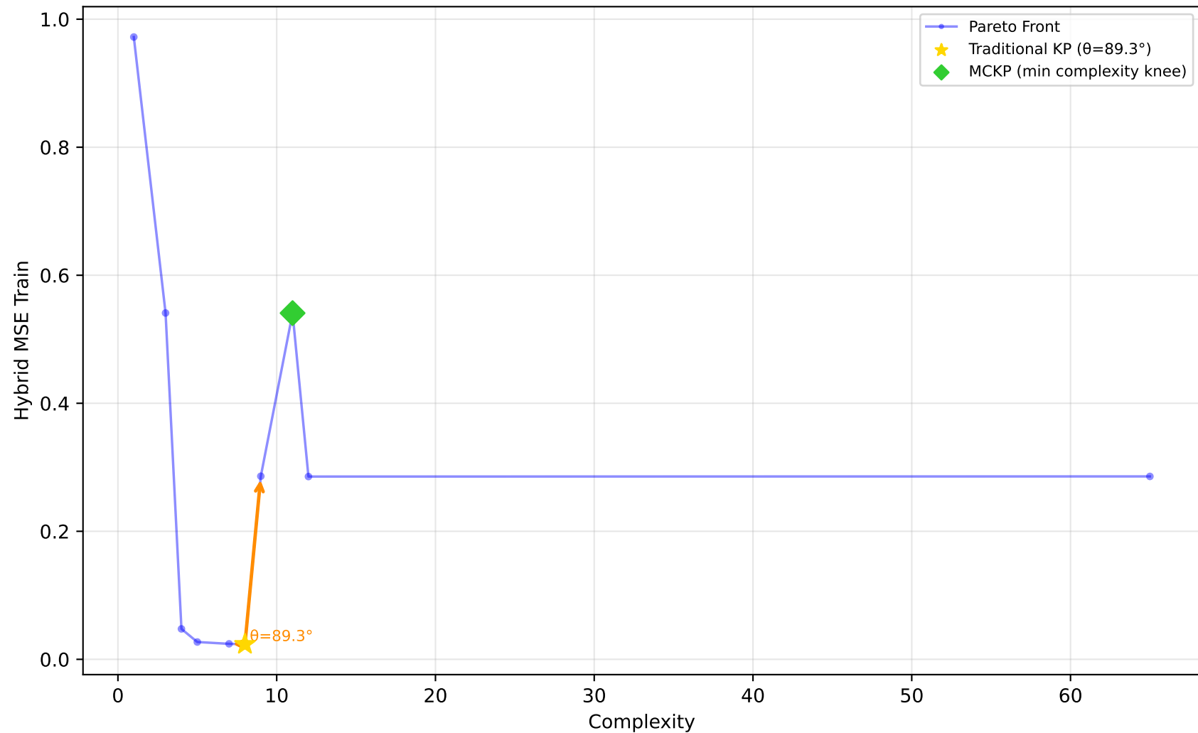
523_analcatdata_neavote - Run 8 - SVP - Hybrid MSE Train \lambda_1=0.00, \lambda_2=0.90, \lambda_3=0.00 | Difficulty: 1.00 | Method: hmr
