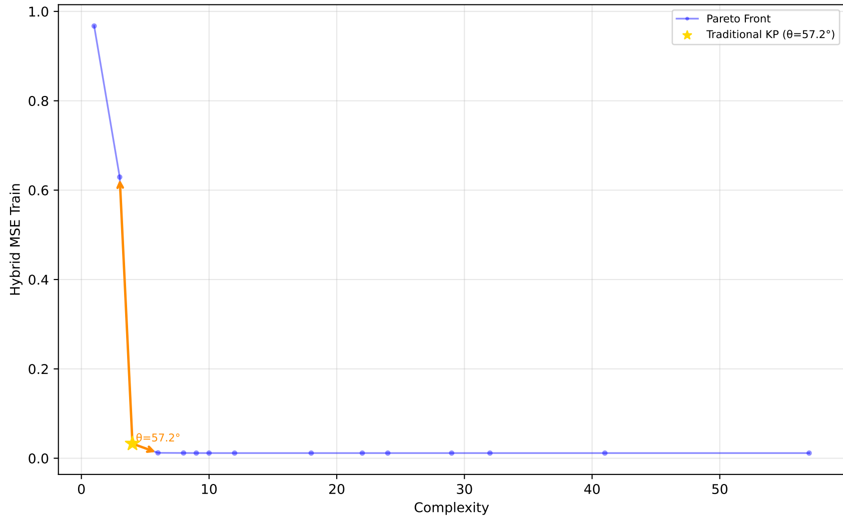
523_analcatdata_neavote - Run 9 - MVP - Hybrid MSE Train \lambda_1=0.00, \lambda_2=0.10, \lambda_3=0.00 | Difficulty: 1.00 | Method: hmr
