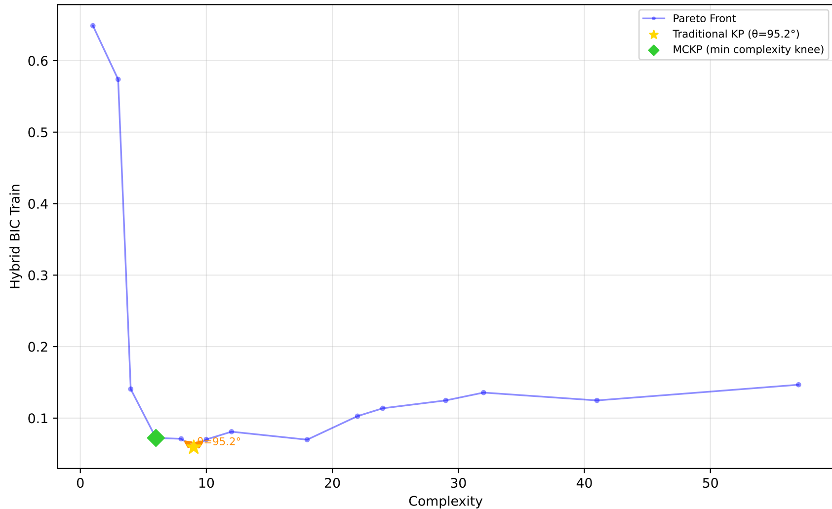
523_analcatdata_neavote - Run 9 - SVP - Hybrid BIC Train \lambda_1=0.00, \lambda_2=0.20, \lambda_3=0.00 | Difficulty: 1.00 | Method: hmr
