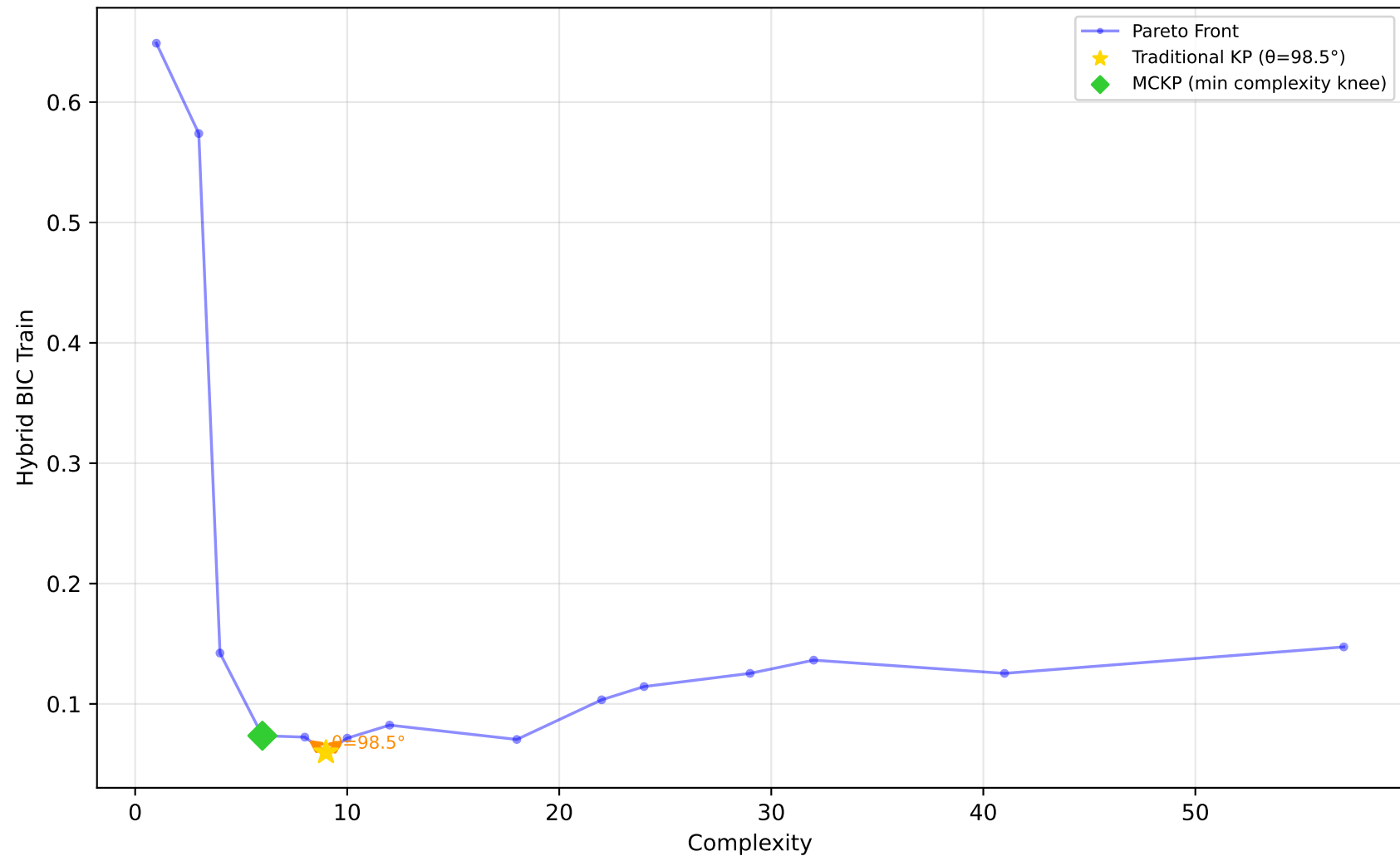
523_analcatdata_neavote - Run 9 - SVP - Hybrid BIC Train \lambda_1=0.00, \lambda_2=0.90, \lambda_3=0.00 | Difficulty: 1.00 | Method: hmr
