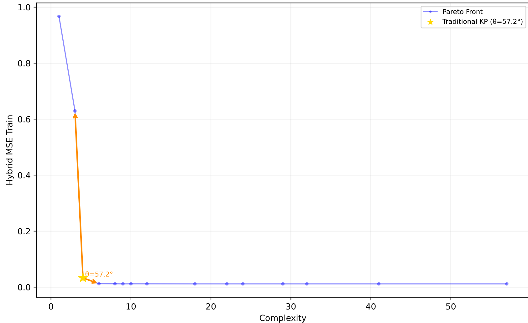
523_analcatdata_neavote - Run 9 - SVP - Hybrid MSE Train \lambda_1=0.00, \lambda_2=0.20, \lambda_3=0.00 | Difficulty: 1.00 | Method: hmr
