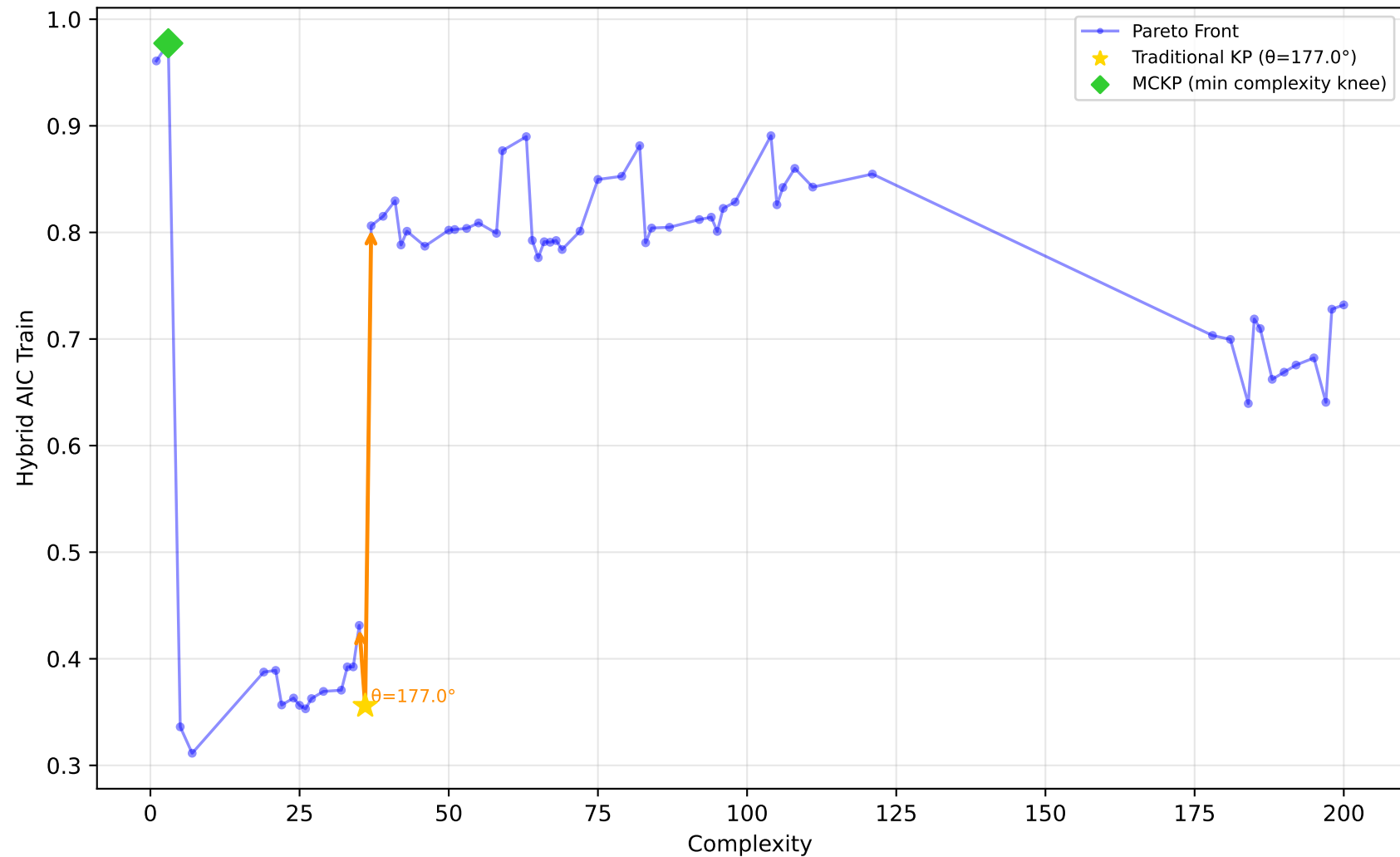
712_chscase_geyser1 - Run 10 - MVP - Hybrid AIC Train \lambda_1=1.00 , \lambda_2=1.00 , \lambda_3=1.00 | Difficulty: 0.90 | Method: hmr
