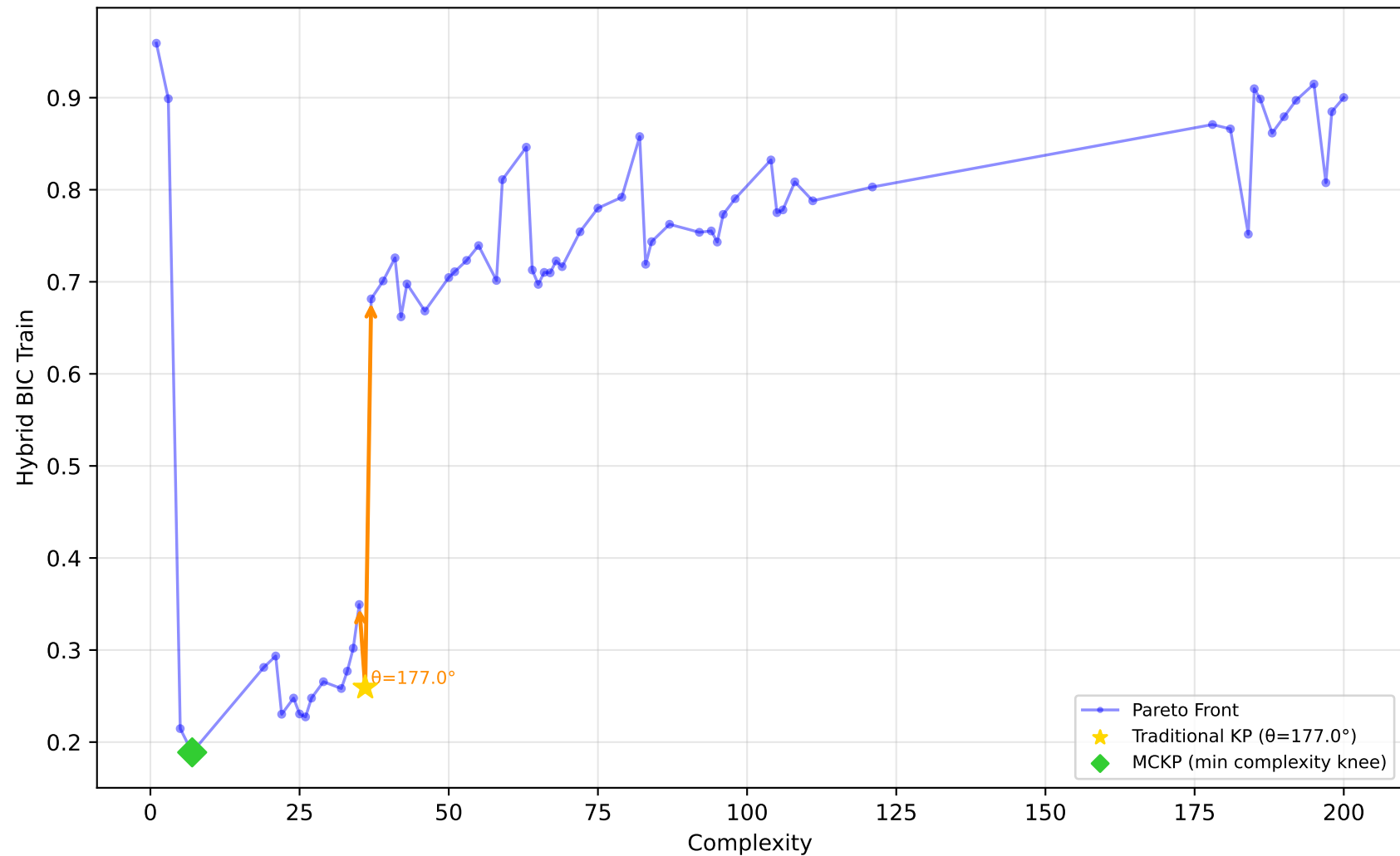
712_chscase_geyser1 - Run 10 - MVP - Hybrid BIC Train \lambda_1=0.20, \lambda_2=1.00, \lambda_3=1.00 | Difficulty: 0.90 | Method: hmr
