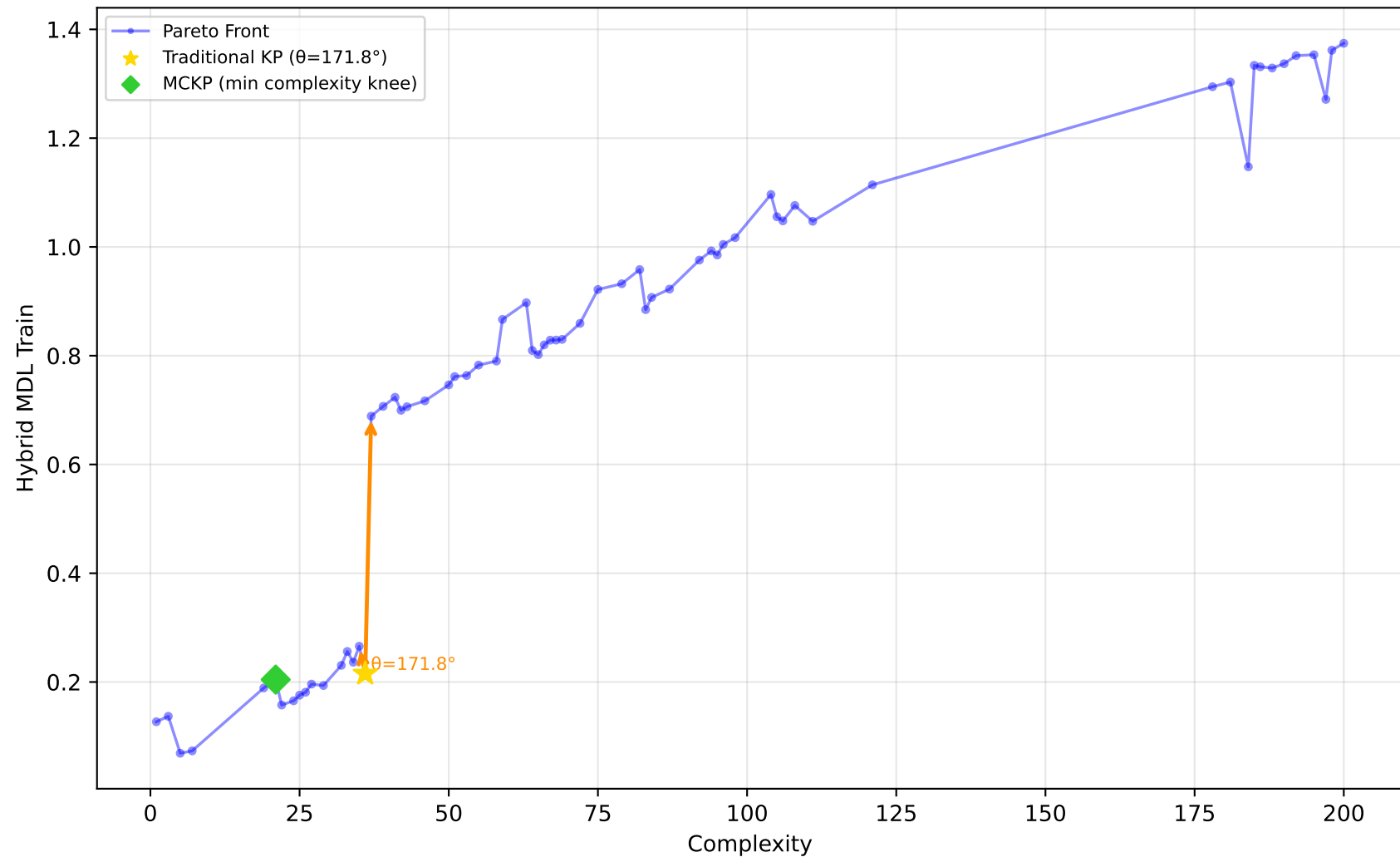
712_chscase_geyser1 - Run 10 - MVP - Hybrid MDL Train \lambda_1=0.20 , \lambda_2=1.00 , \lambda_3=1.00 | Difficulty: 0.90 | Method: hmr
