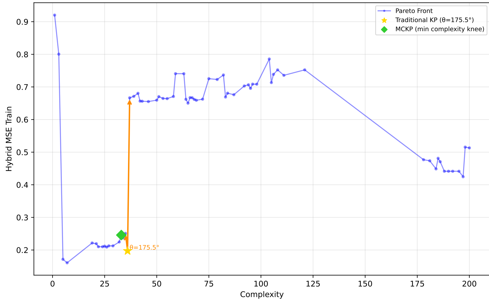
712_chscase_geyser1 - Run 10 - MVP - Hybrid MSE Train \lambda_1=0.20, \lambda_2=1.00, \lambda_3=1.00 | Difficulty: 0.90 | Method: hmr
