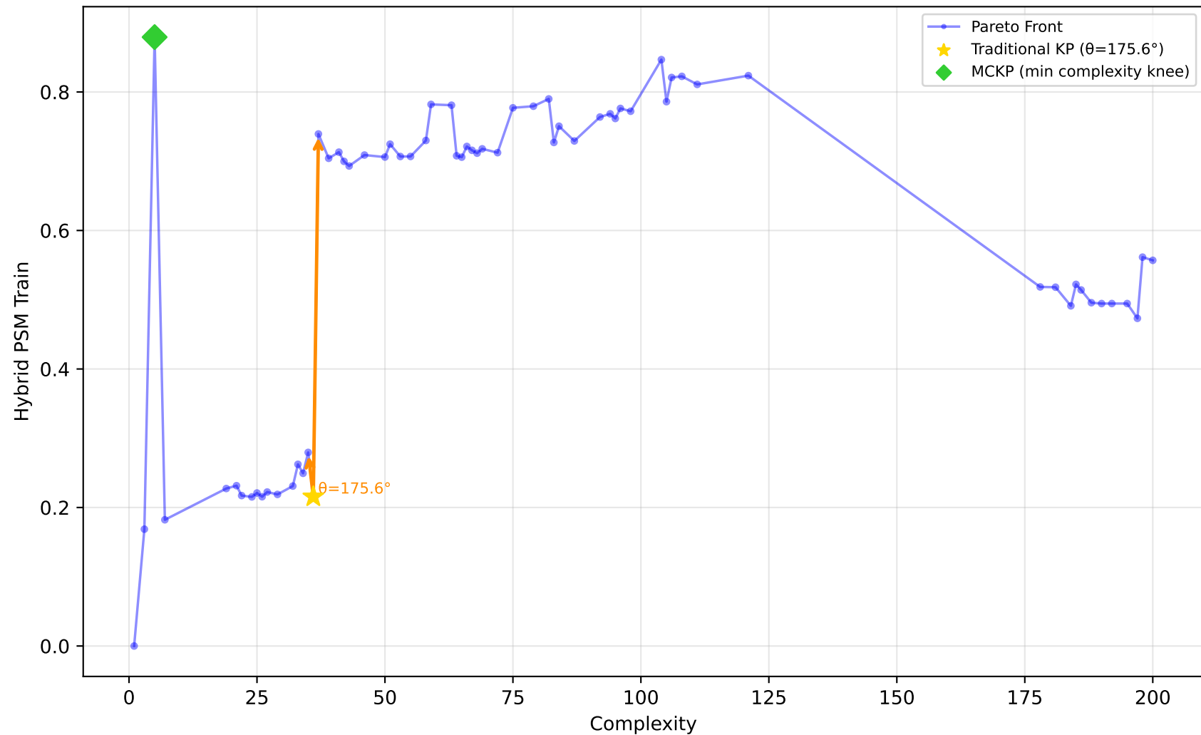
712_chscase_geyser1 - Run 10 - MVP - Hybrid PSM Train \lambda_1=1.00, \lambda_2=1.00, \lambda_3=1.00 | Difficulty: 0.90 | Method: hmr
