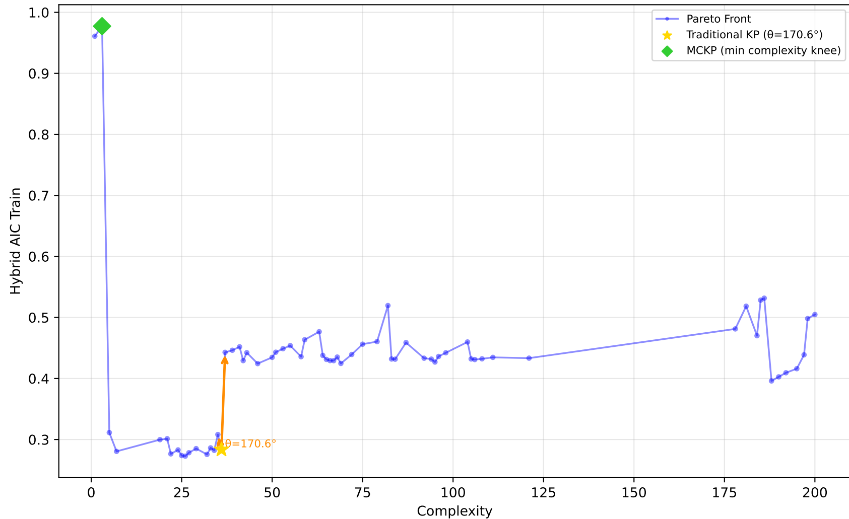
712_chscase_geyser1 - Run 10 - SVP - Hybrid AIC Train \lambda_1=1.00, \lambda_2=1.00, \lambda_3=0.00 | Difficulty: 0.90 | Method: hmr
