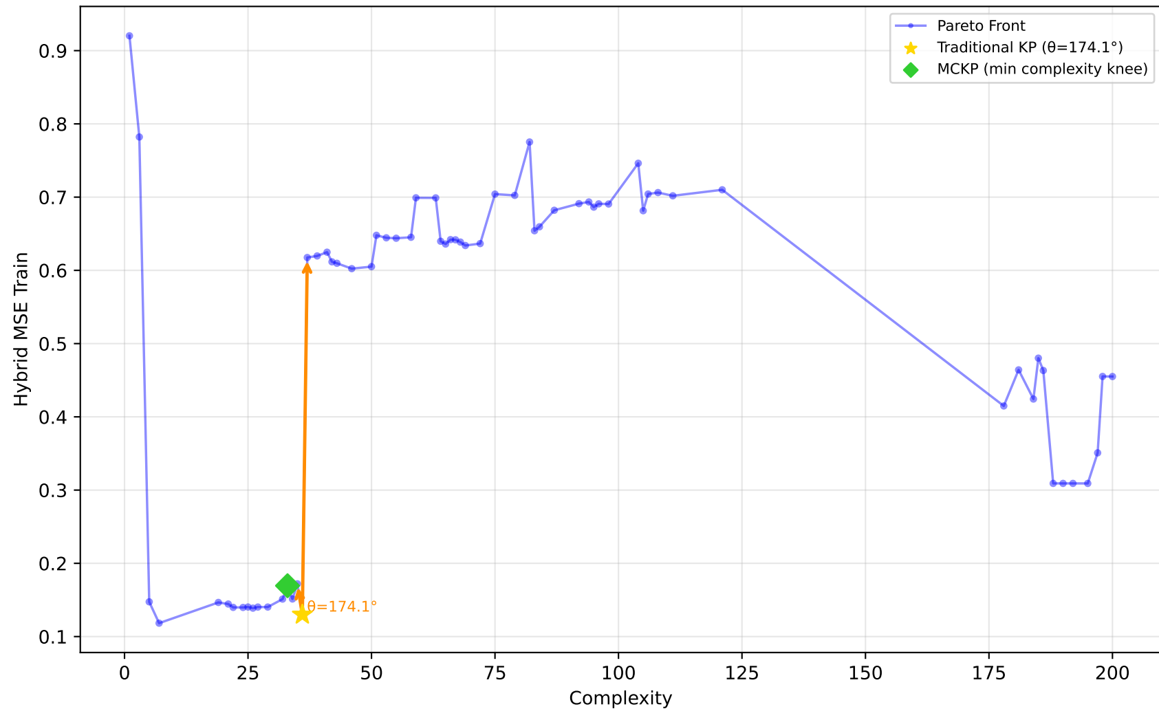
712_chscase_geyser1 - Run 10 - SVP - Hybrid MSE Train \lambda_1=0.00, \lambda_2=1.00, \lambda_3=1.00 | Difficulty: 0.90 | Method: hmr
