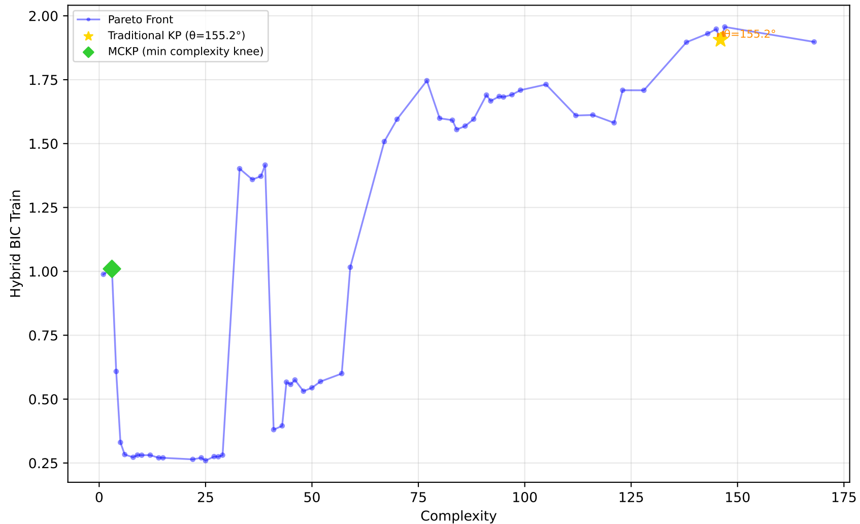
712_chscase_geyser1 - Run 11 - MVP - Hybrid BIC Train \lambda_1=1.00 , \lambda_2=1.00 , \lambda_3=1.00 | Difficulty: 1.00 | Method: hmr
