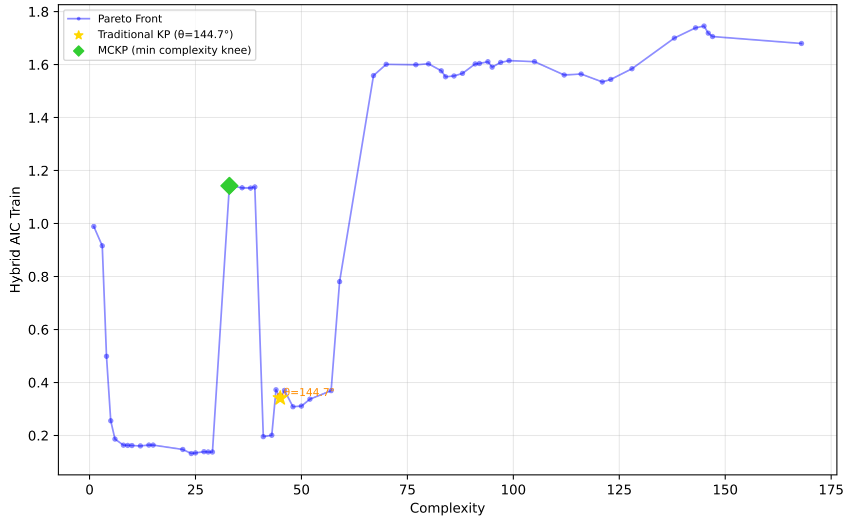
712_chscase_geyser1 - Run 11 - SVP - Hybrid AIC Train \lambda_1=0.00 , \lambda_2=1.00 , \lambda_3=1.00 | Difficulty: 1.00 | Method: hmr
