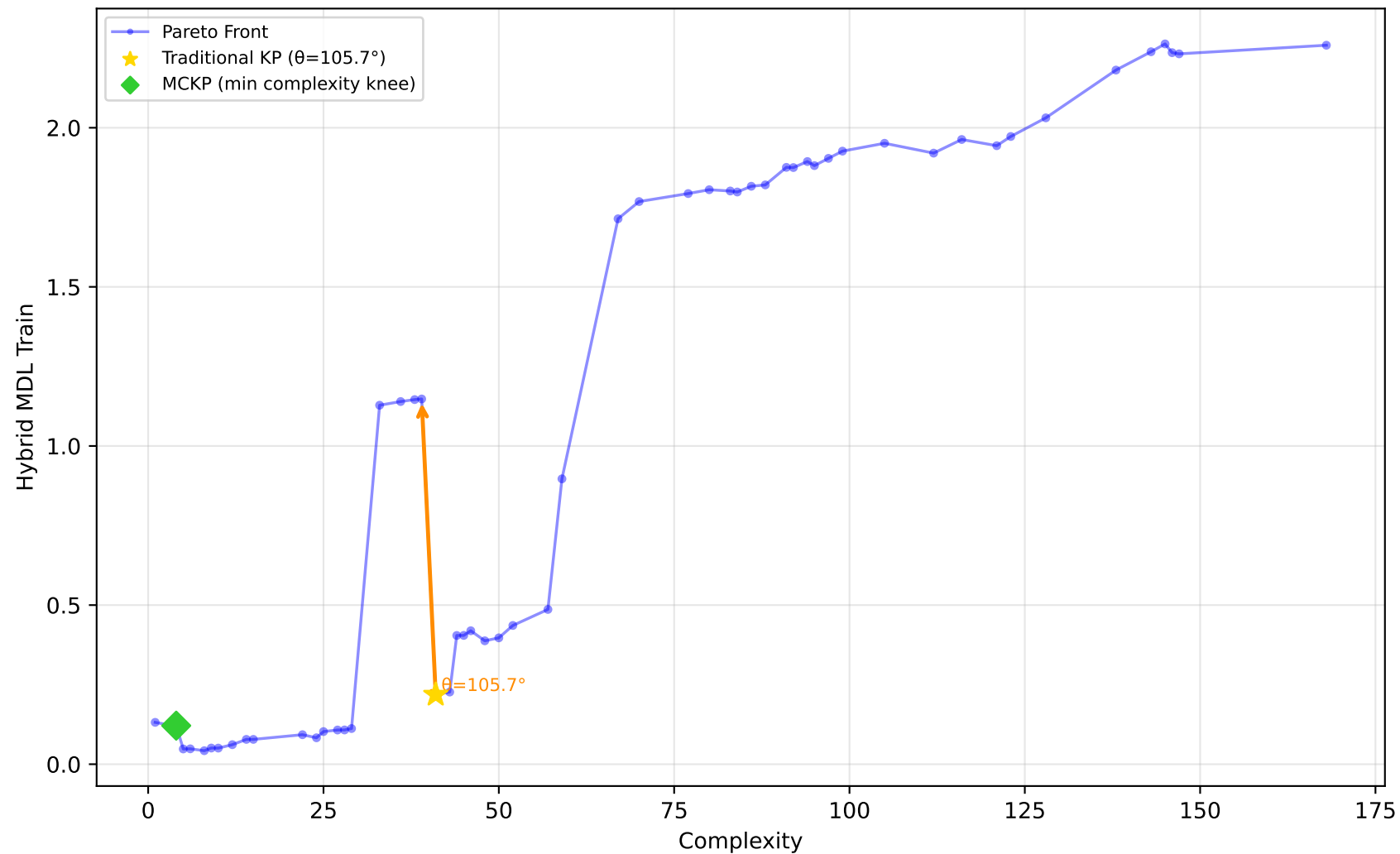
712_chscase_geyser1 - Run 11 - SVP - Hybrid MDL Train \lambda_1=0.00 , \lambda_2=1.00 , \lambda_3=1.00 | Difficulty: 1.00 | Method: hmr
