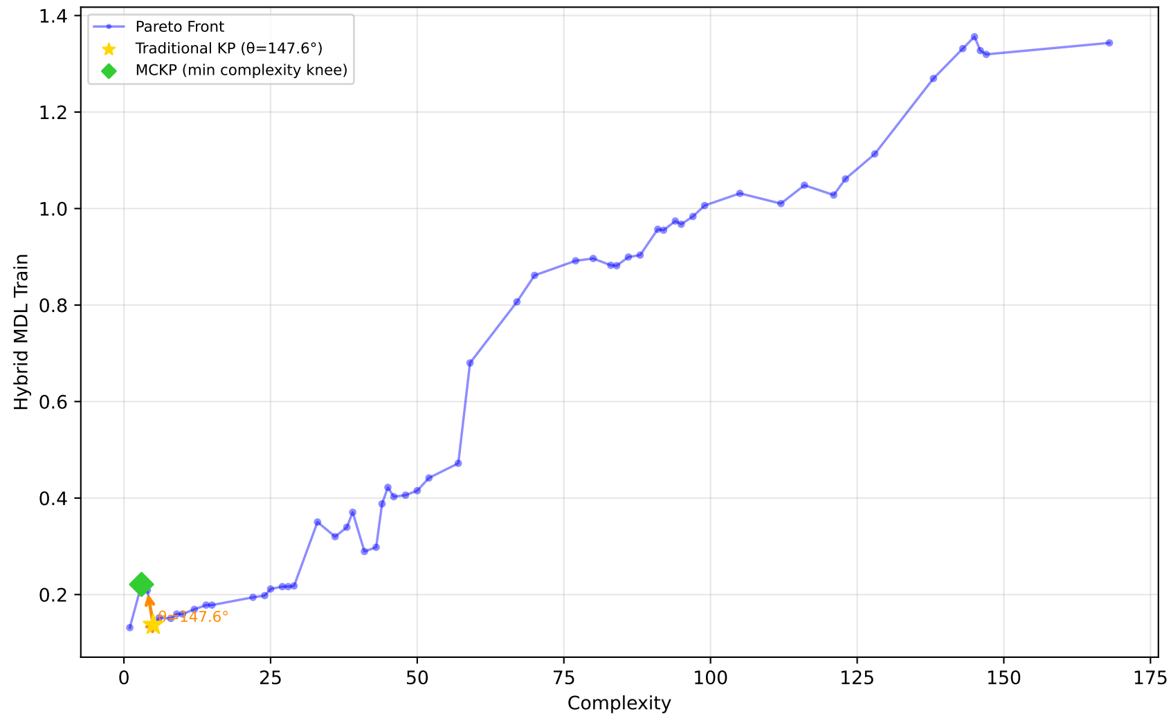
712_chscase_geyser1 - Run 11 - SVP - Hybrid MDL Train \lambda_1=1.00, \lambda_2=1.00, \lambda_3=0.00 | Difficulty: 1.00 | Method: hmr
