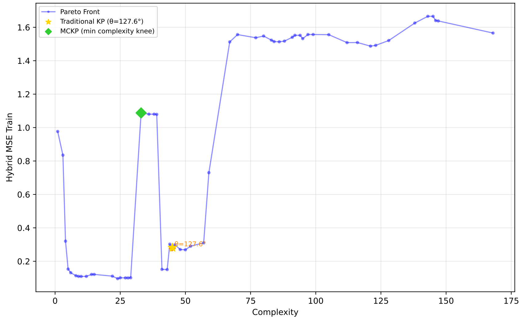
712_chscase_geyser1 - Run 11 - SVP - Hybrid MSE Train \lambda_1=0.00, \lambda_2=1.00, \lambda_3=1.00 | Difficulty: 1.00 | Method: hmr
