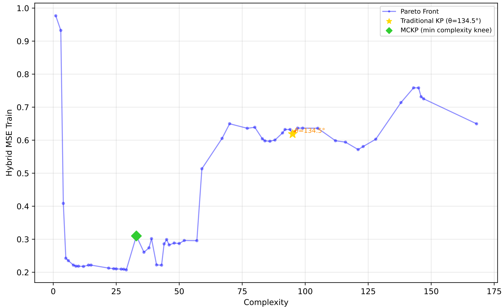
712_chscase_geyser1 - Run 11 - SVP - Hybrid MSE Train \lambda_1=1.00, \lambda_2=1.00, \lambda_3=0.00 | Difficulty: 1.00 | Method: hmr
