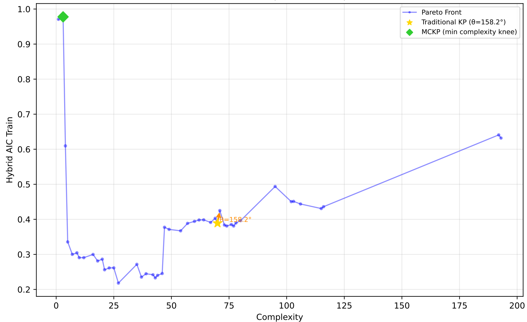
712_chscase_geyser1 - Run 12 - MVP - Hybrid AIC Train \lambda_1=1.00, \lambda_2=1.00, \lambda_3=1.00 | Difficulty: 0.66 | Method: hmr
