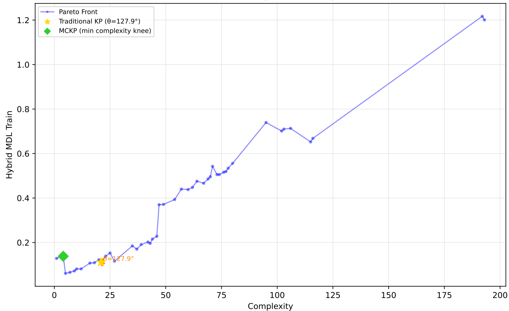
712_chscase_geyser1 - Run 12 - MVP - Hybrid MDL Train \lambda_1=0.20, \lambda_2=1.00, \lambda_3=1.00 | Difficulty: 0.66 | Method: hmr
