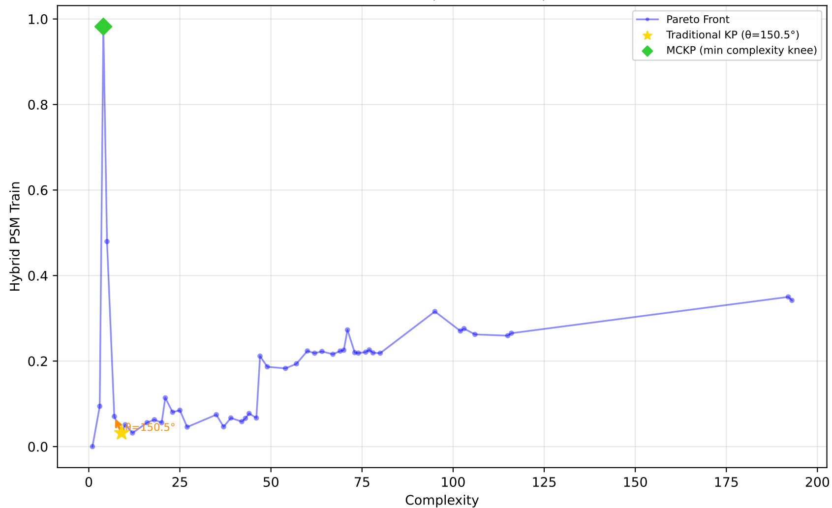
712_chscase_geyser1 - Run 12 - MVP - Hybrid PSM Train \lambda_1=0.20, \lambda_2=1.00, \lambda_3=1.00 | Difficulty: 0.66 | Method: hmr
