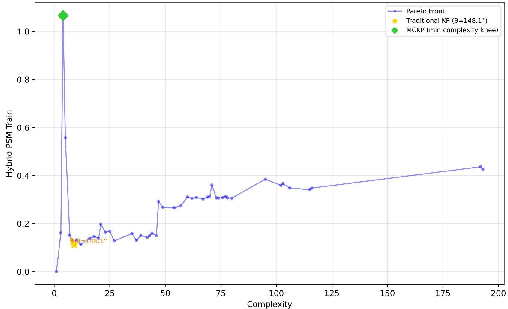
712_chscase_geyser1 - Run 12 - MVP - Hybrid PSM Train \lambda_1=1.00, \lambda_2=1.00, \lambda_3=1.00 | Difficulty: 0.66 | Method: hmr
