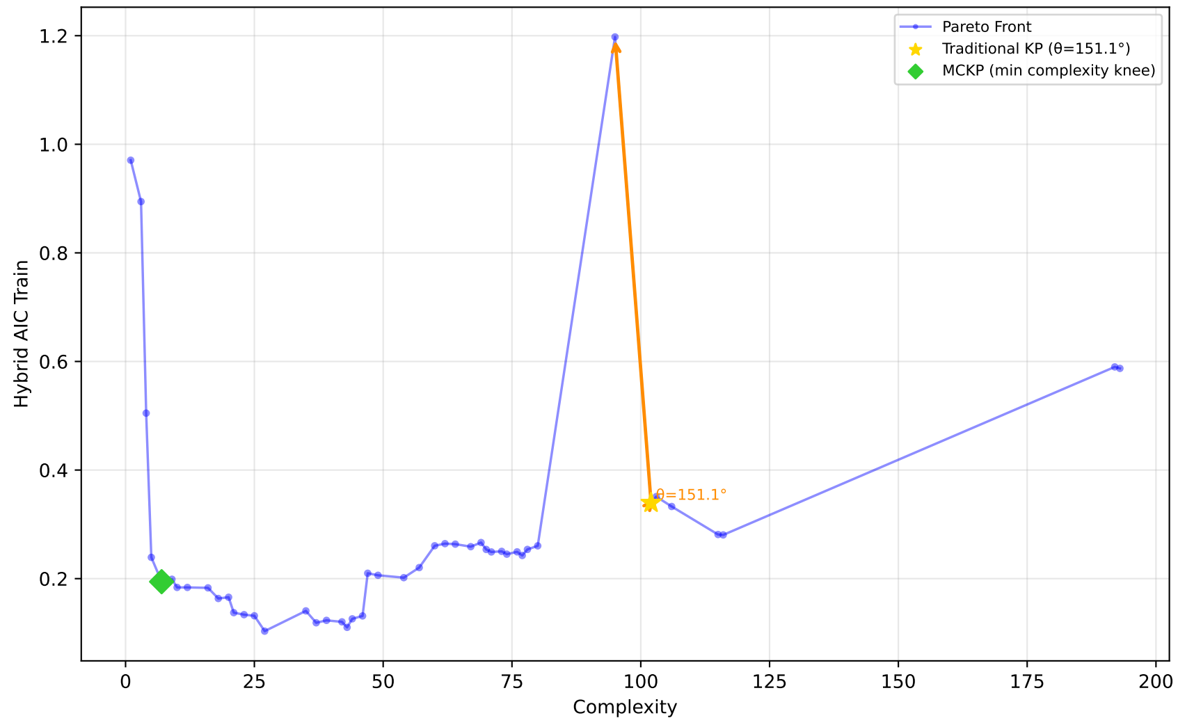
712_chscase_geyser1 - Run 12 - SVP - Hybrid AIC Train \lambda_1=0.00 , \lambda_2=1.00 , \lambda_3=1.00 | Difficulty: 0.66 | Method: hmr
