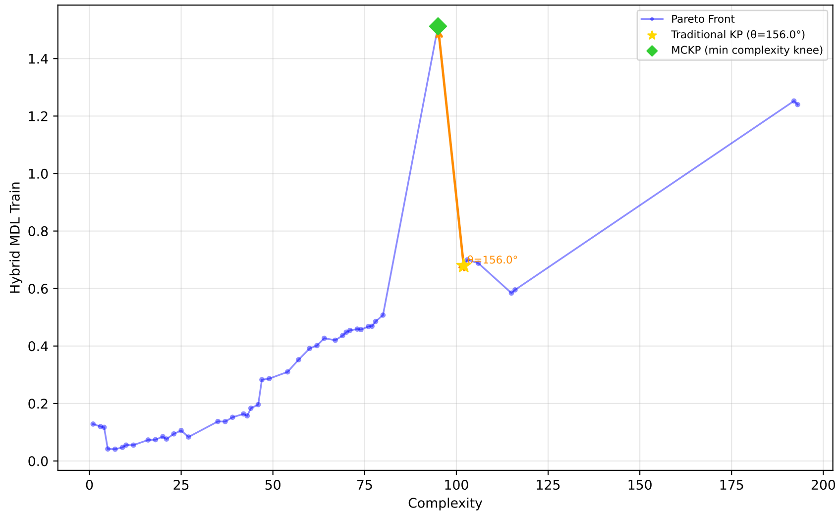
712_chscase_geyser1 - Run 12 - SVP - Hybrid MDL Train \lambda_1=0.00 , \lambda_2=1.00 , \lambda_3=1.00 | Difficulty: 0.66 | Method: hmr
