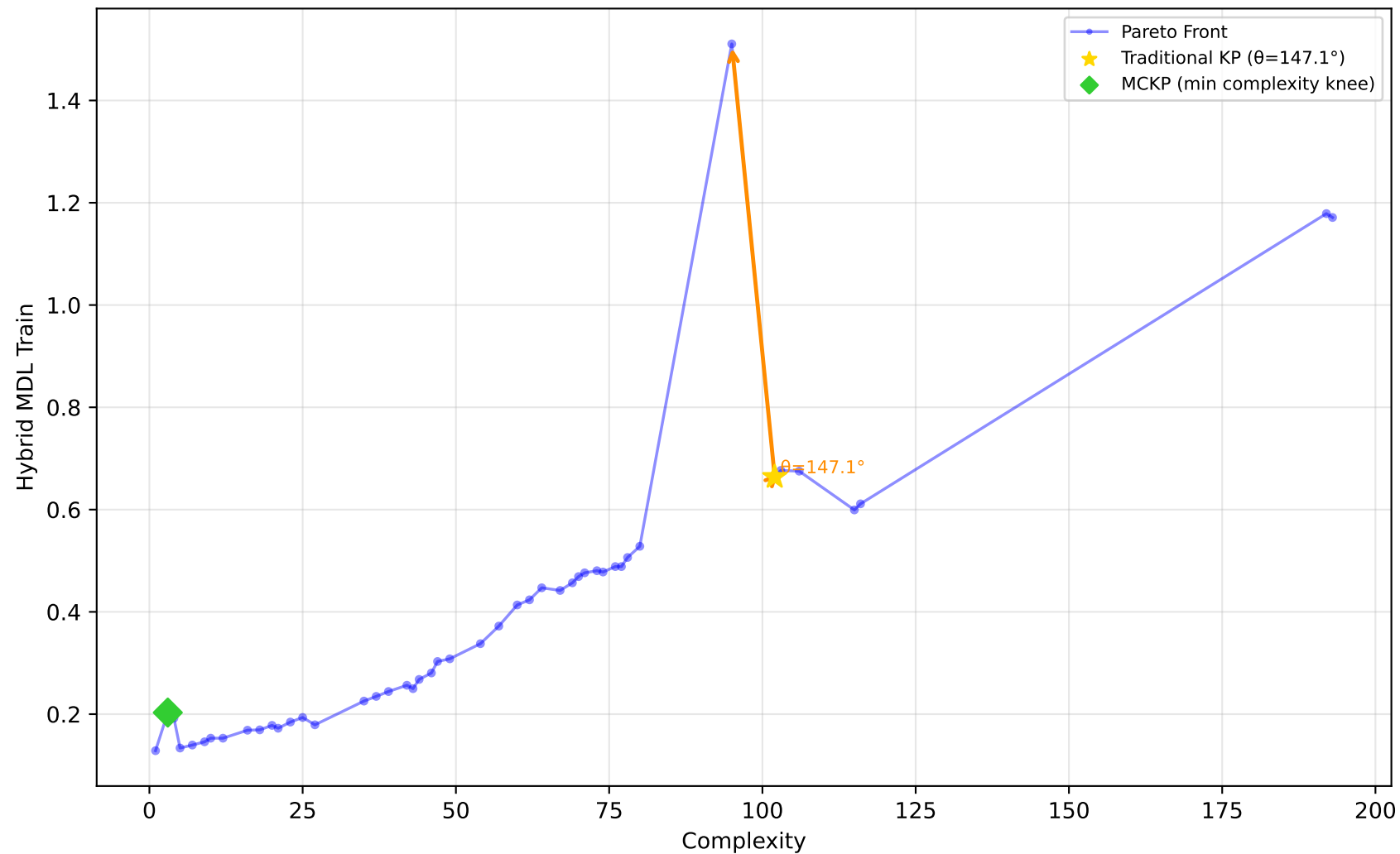
712_chscase_geyser1 - Run 12 - SVP - Hybrid MDL Train \lambda_1=1.00, \lambda_2=1.00, \lambda_3=0.00 | Difficulty: 0.66 | Method: hmr
