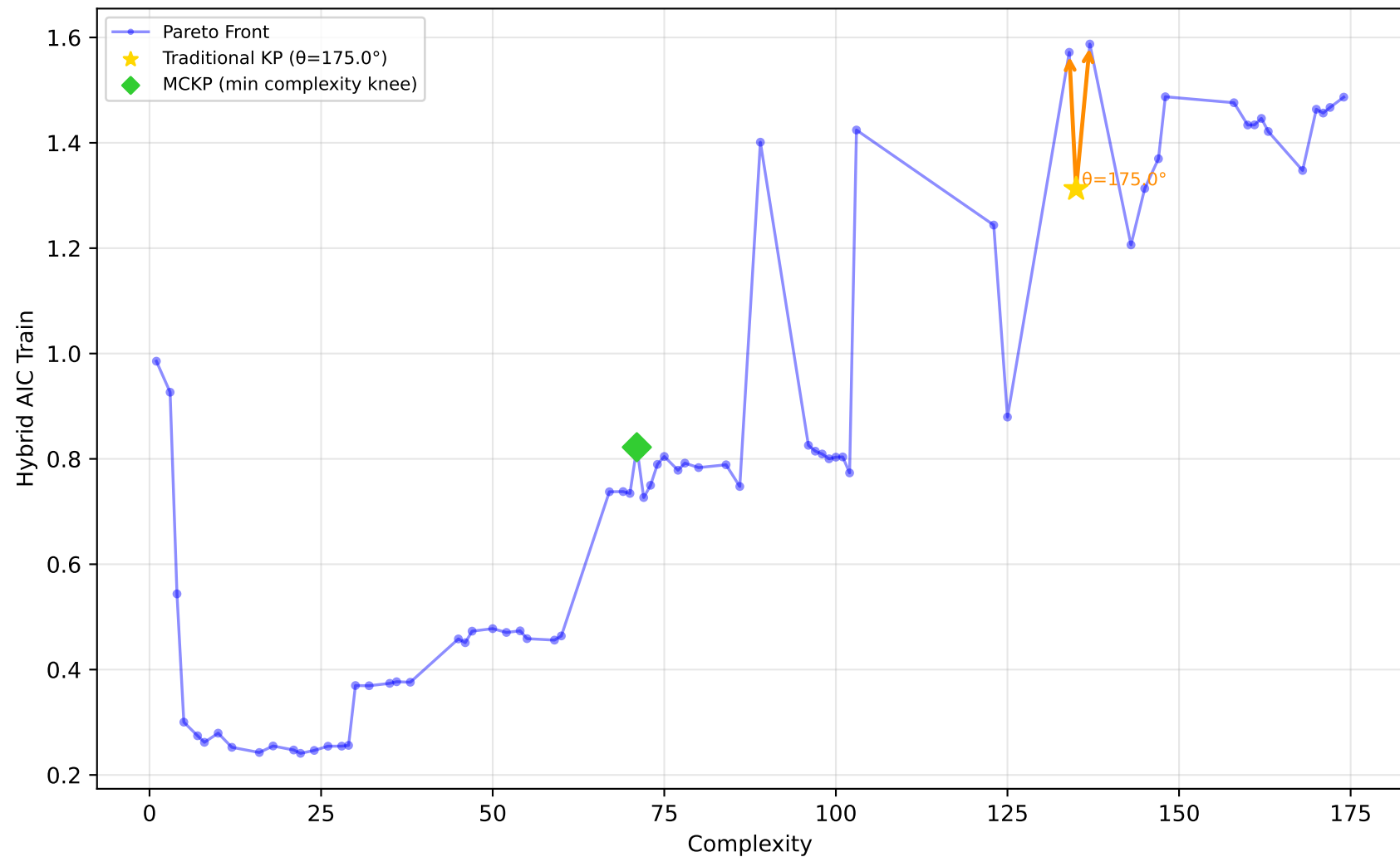
712_chscase_geyser1 - Run 13 - MVP - Hybrid AIC Train \lambda_1=0.20 , \lambda_2=1.00 , \lambda_3=1.00 | Difficulty: 0.48 | Method: mckp
