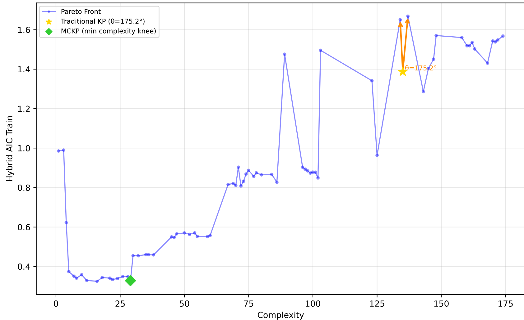
712_chscase_geyser1 - Run 13 - MVP - Hybrid AIC Train \lambda_1=1.00, \lambda_2=1.00, \lambda_3=1.00 | Difficulty: 0.48 | Method: mckp
