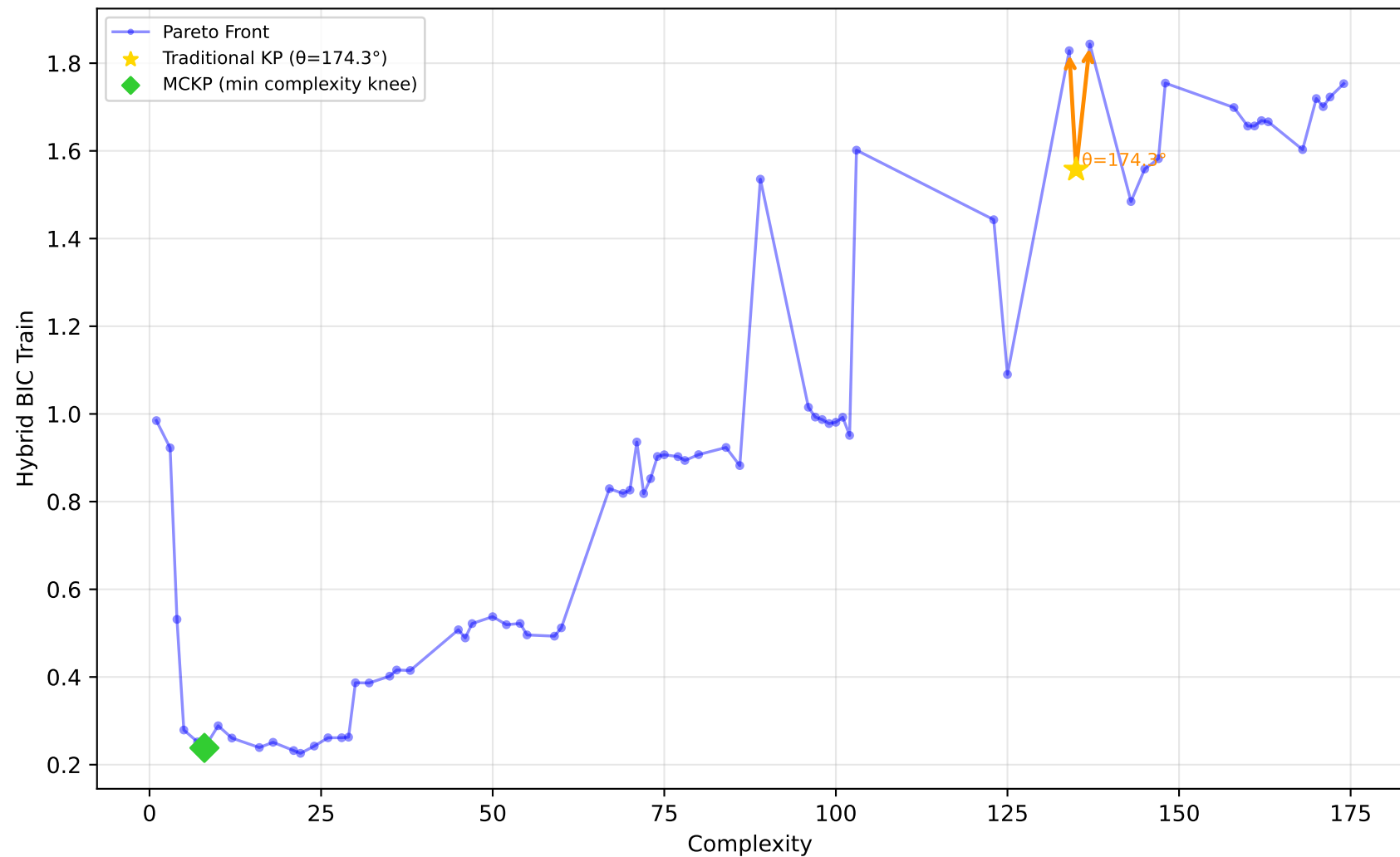
712_chscase_geyser1 - Run 13 - MVP - Hybrid BIC Train \lambda_1=0.20, \lambda_2=1.00, \lambda_3=1.00 | Difficulty: 0.48 | Method: mckp
