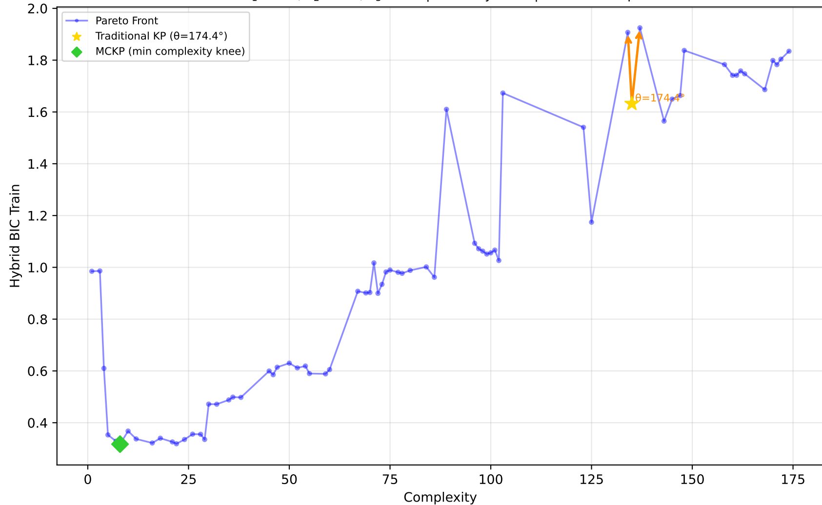
712_chscase_geyser1 - Run 13 - MVP - Hybrid BIC Train \lambda_1=1.00, \lambda_2=1.00, \lambda_3=1.00 | Difficulty: 0.48 | Method: mckp
