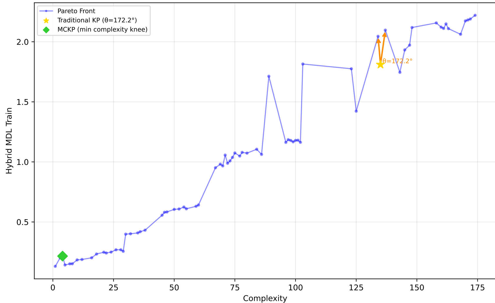
712_chscase_geyser1 - Run 13 - MVP - Hybrid MDL Train \lambda_1=1.00, \lambda_2=1.00, \lambda_3=1.00 | Difficulty: 0.48 | Method: mckp
