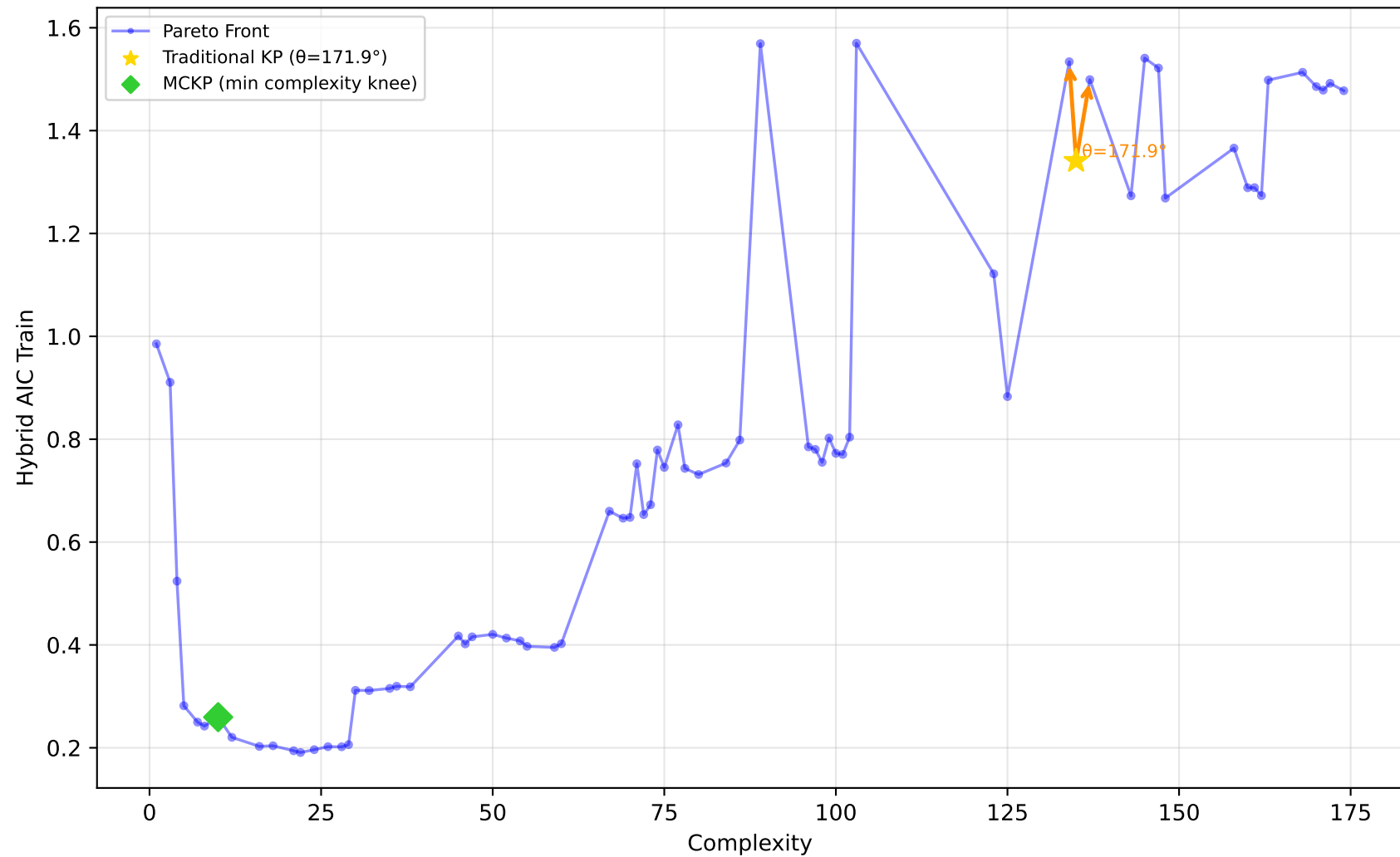
712_chscase_geyser1 - Run 13 - SVP - Hybrid AIC Train \lambda_1=0.00 , \lambda_2=1.00 , \lambda_3=1.00 | Difficulty: 0.48 | Method: mckp
