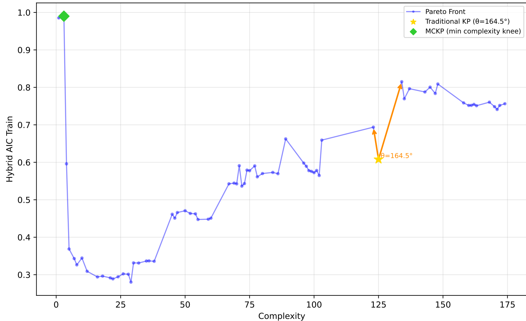
712_chscase_geyser1 - Run 13 - SVP - Hybrid AIC Train \lambda_1=1.00 , \lambda_2=1.00 , \lambda_3=0.00 | Difficulty: 0.48 | Method: mckp
