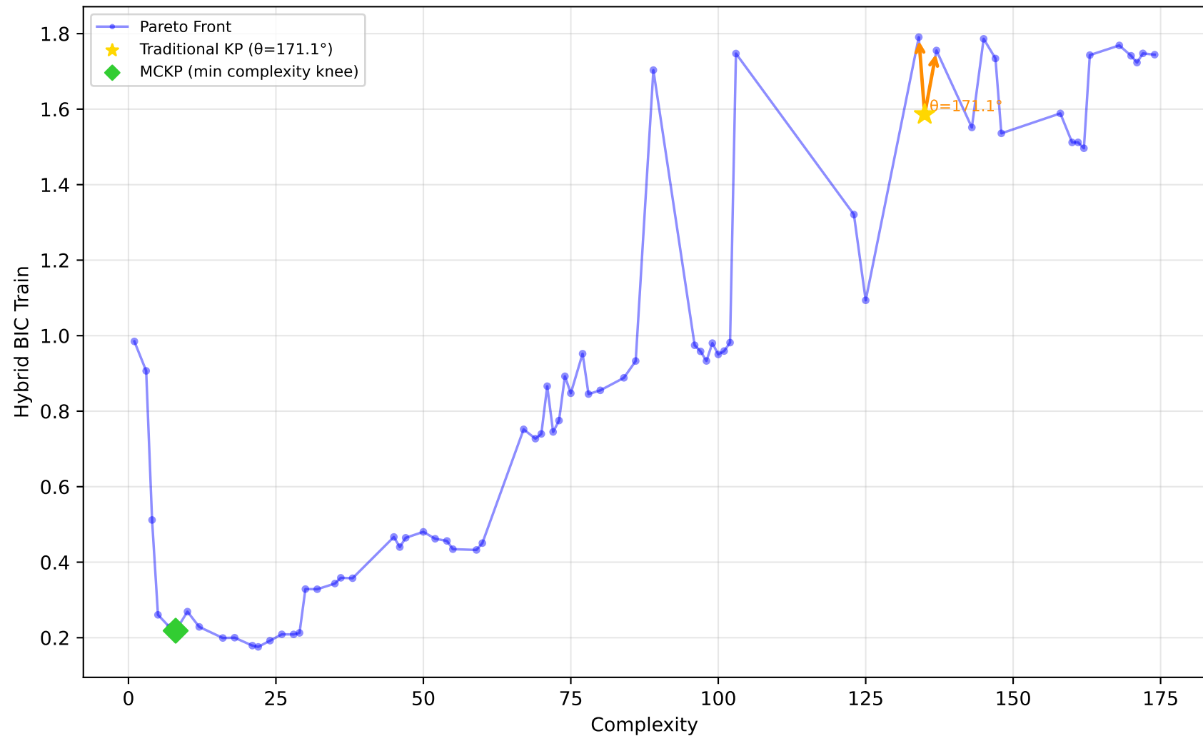
712_chscase_geyser1 - Run 13 - SVP - Hybrid BIC Train \lambda_1=0.00, \lambda_2=1.00, \lambda_3=1.00 | Difficulty: 0.48 | Method: mckp
