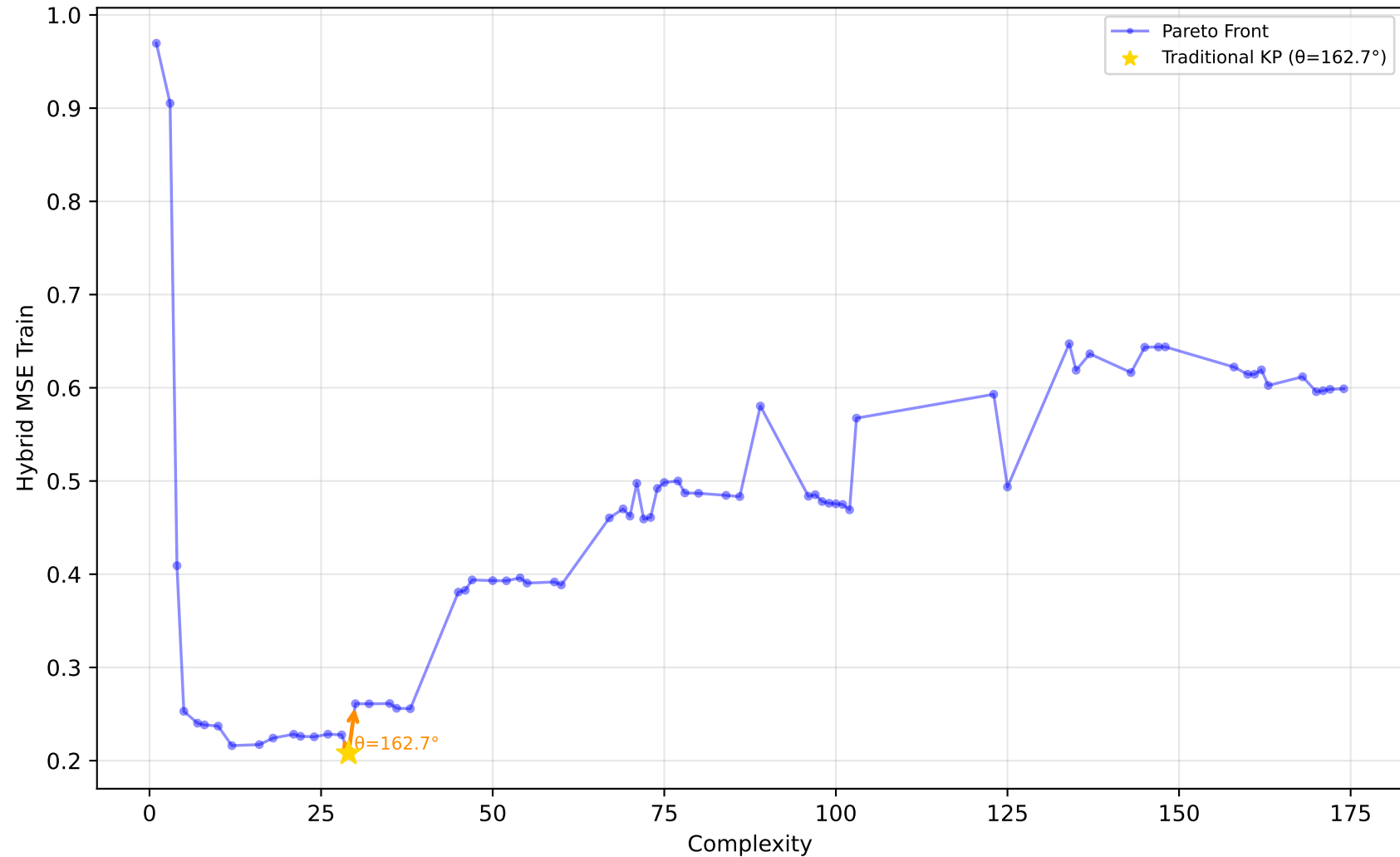
712_chscase_geyser1 - Run 13 - SVP - Hybrid MSE Train \lambda_1=1.00, \lambda_2=1.00, \lambda_3=0.00 | Difficulty: 0.48 | Method: mckp
