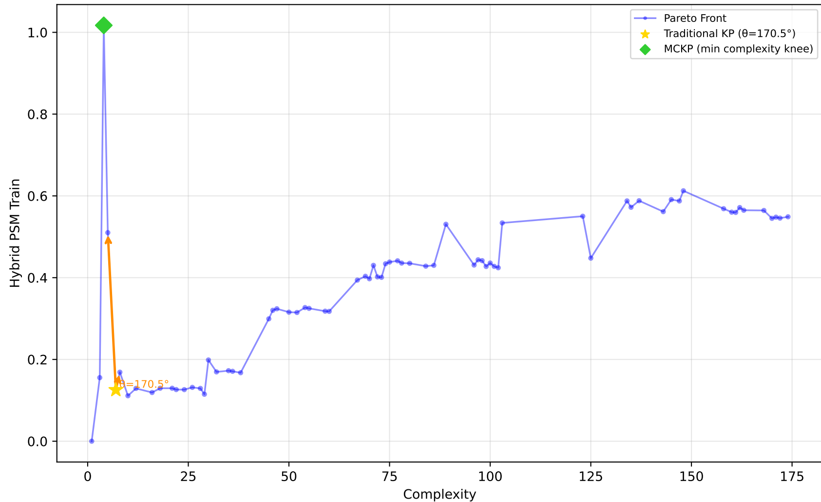
712_chscase_geyser1 - Run 13 - SVP - Hybrid PSM Train \lambda_1=1.00, \lambda_2=1.00, \lambda_3=0.00 | Difficulty: 0.48 | Method: mckp
