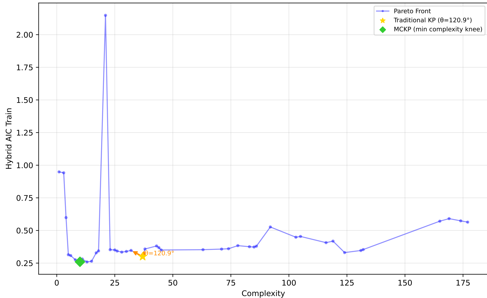
712_chscase_geyser1 - Run 14 - MVP - Hybrid AIC Train \lambda_1=1.00, \lambda_2=1.00, \lambda_3=1.00 | Difficulty: 0.76 | Method: hmr
