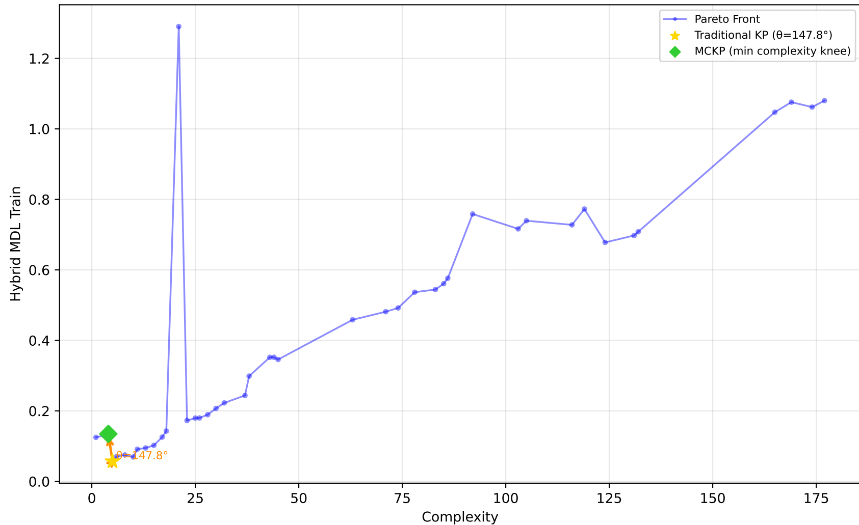
712_chscase_geyser1 - Run 14 - MVP - Hybrid MDL Train \lambda_1=0.20, \lambda_2=1.00, \lambda_3=1.00 | Difficulty: 0.76 | Method: hmr
