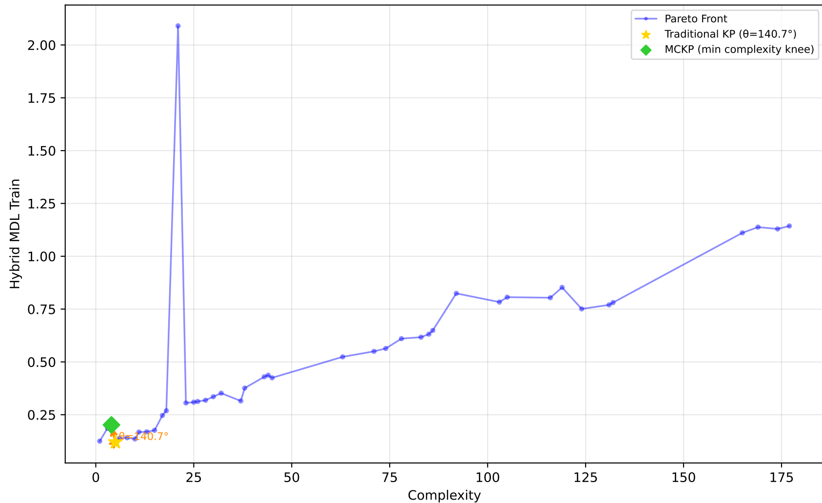
712_chscase_geyser1 - Run 14 - MVP - Hybrid MDL Train \lambda_1=1.00, \lambda_2=1.00, \lambda_3=1.00 | Difficulty: 0.76 | Method: hmr
