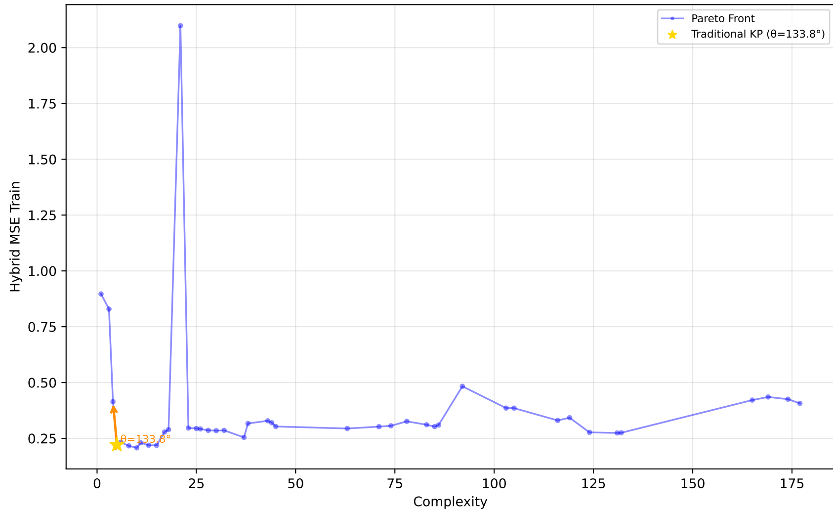
712_chscase_geyser1 - Run 14 - MVP - Hybrid MSE Train \lambda_1=1.00, \lambda_2=1.00, \lambda_3=1.00 | Difficulty: 0.76 | Method: hmr
