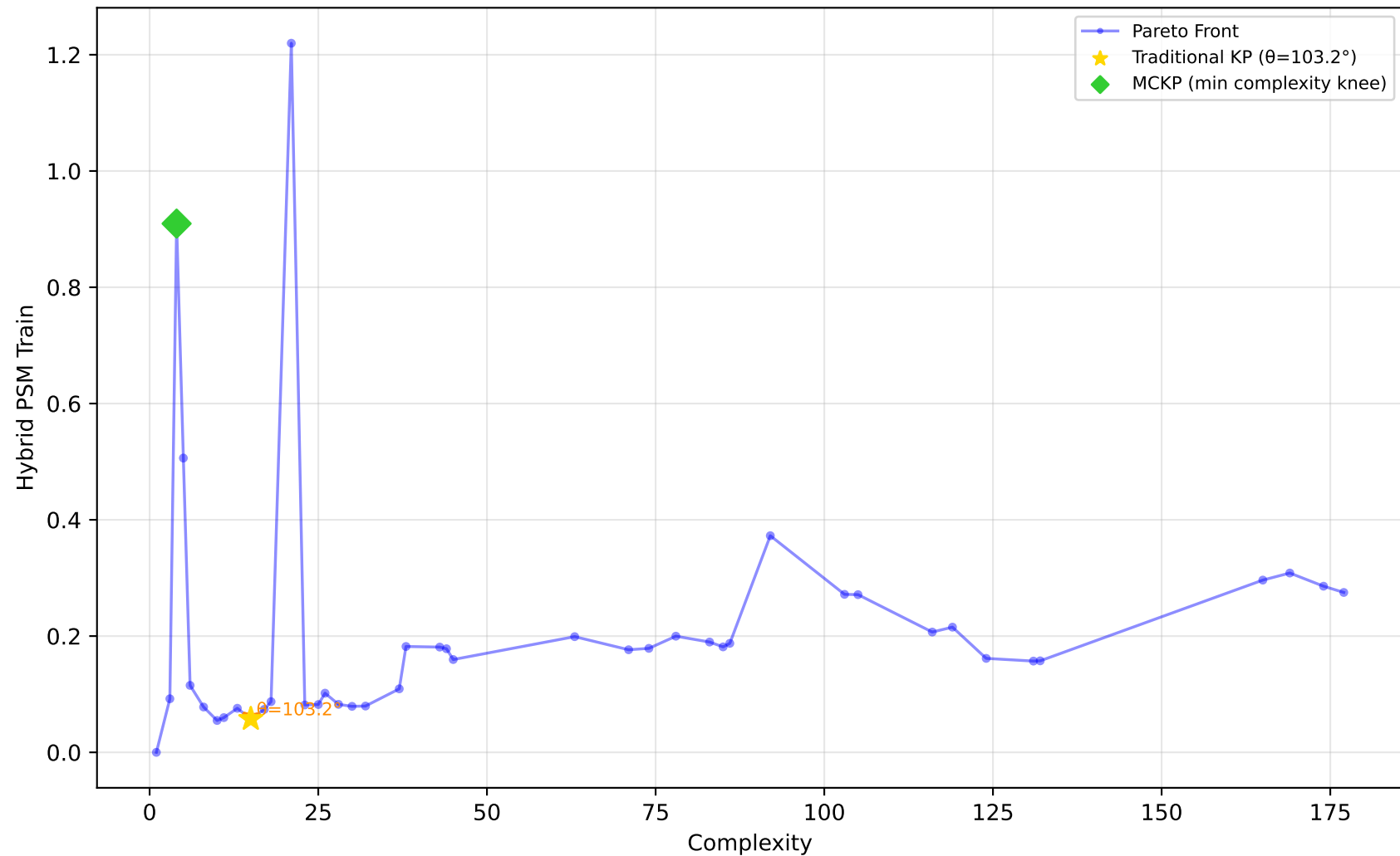
712_chscase_geyser1 - Run 14 - MVP - Hybrid PSM Train \lambda_1=0.20, \lambda_2=1.00, \lambda_3=1.00 | Difficulty: 0.76 | Method: hmr
